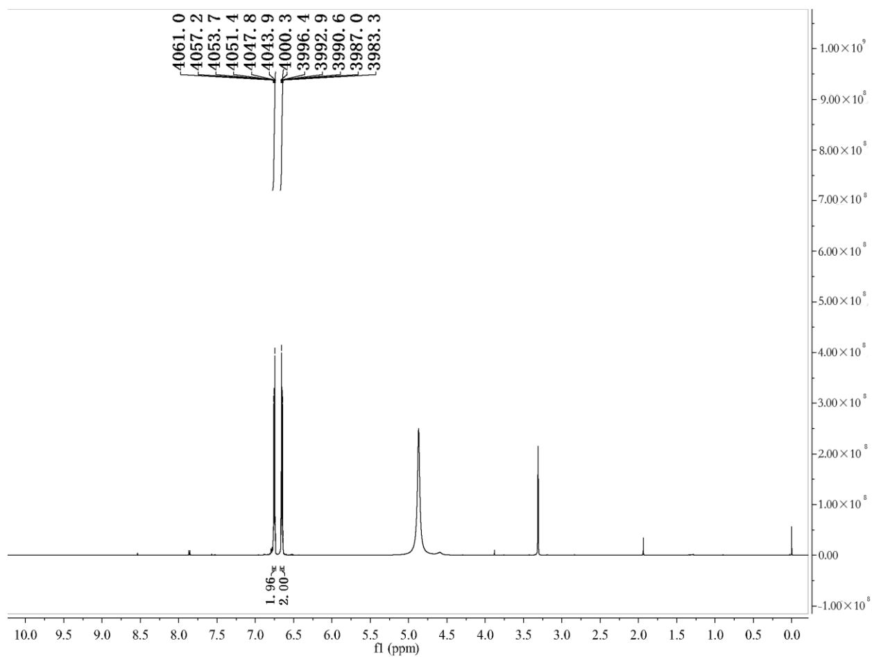
Figure S2. The ^1\text{H} -NMR profile of catechol (The original profile).
