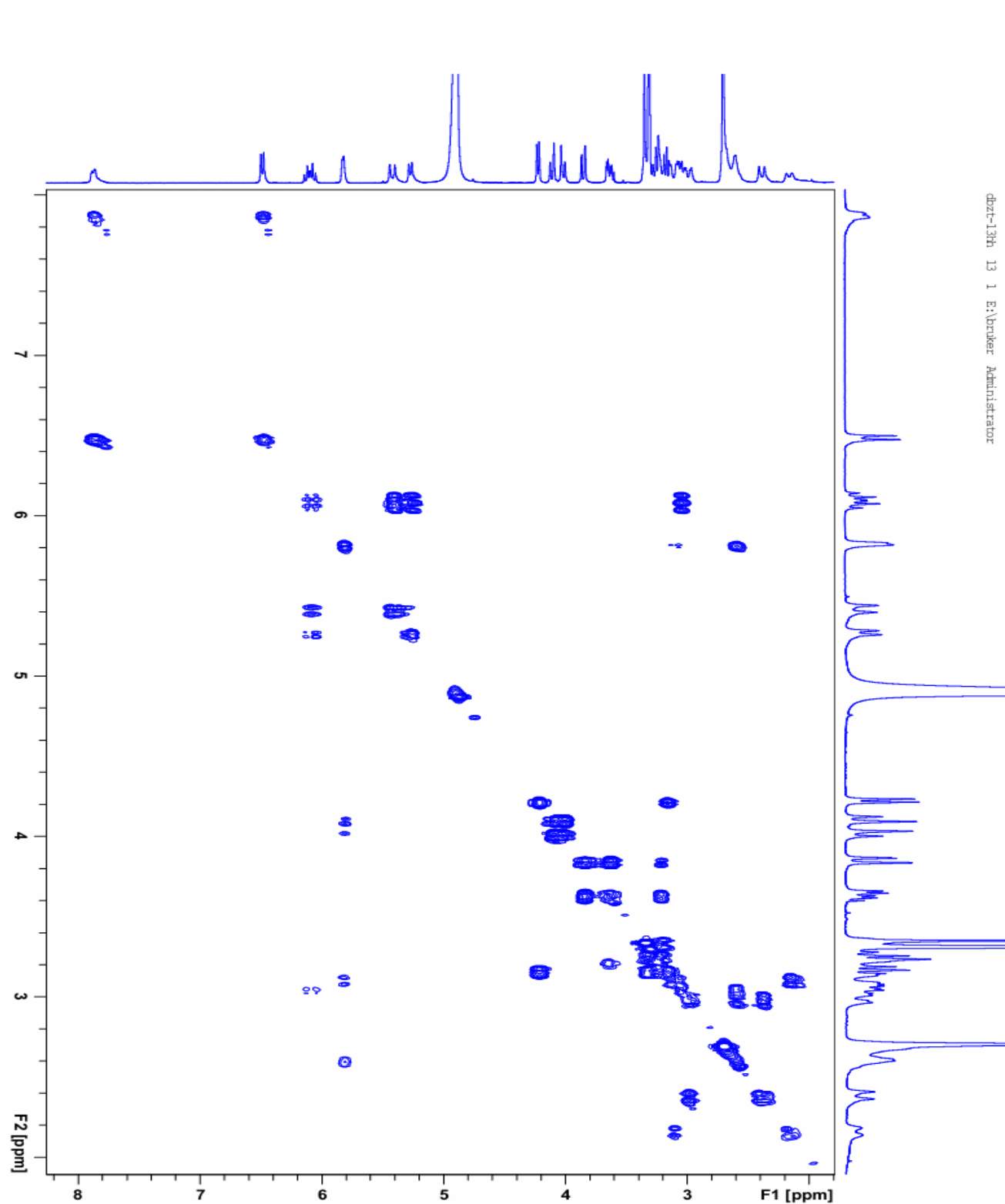
Figure S21. ^1\text{H} - ^1\text{H} COSY spectrum of compound 4 .
