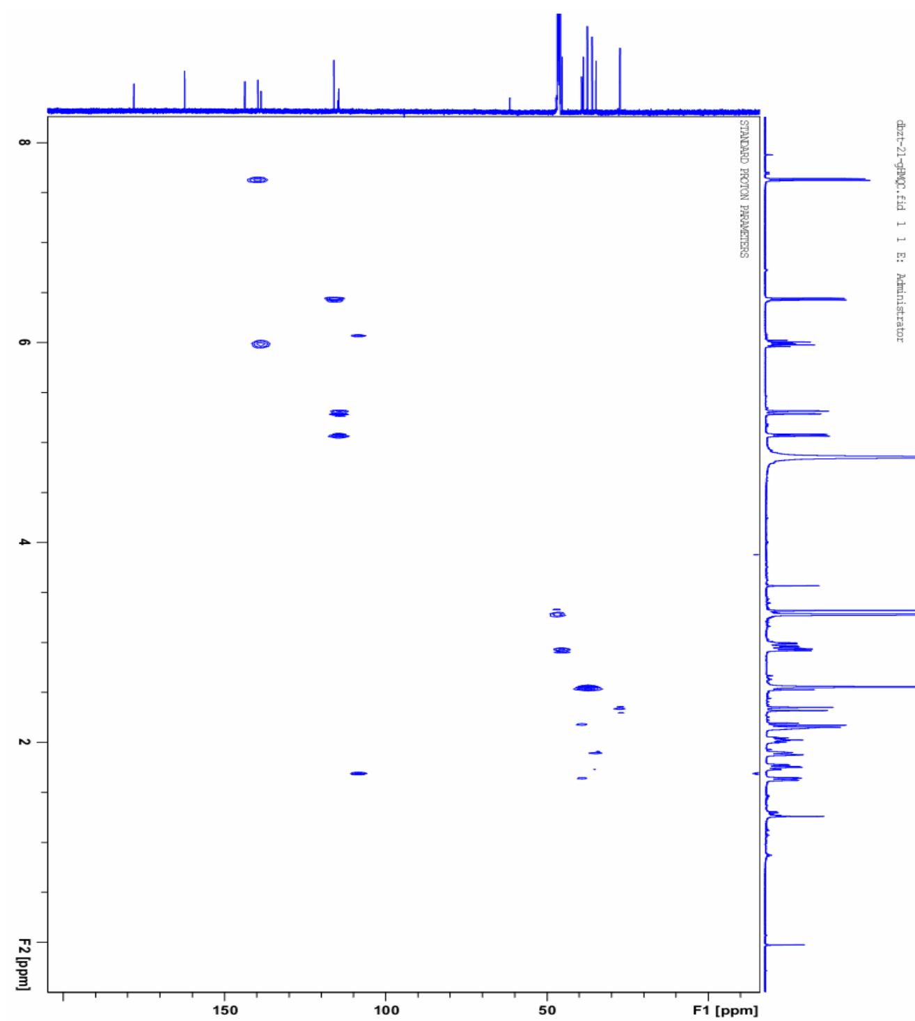
Figure S16. HSQC spectrum of compound 3 .
