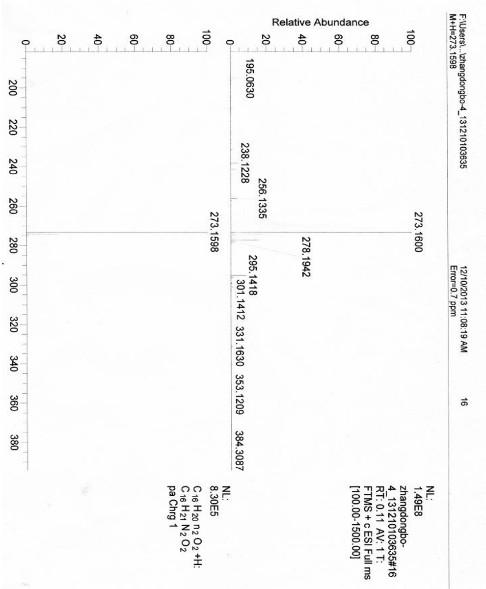
Figure S6. HRESIMS spectrum of compound 1.
