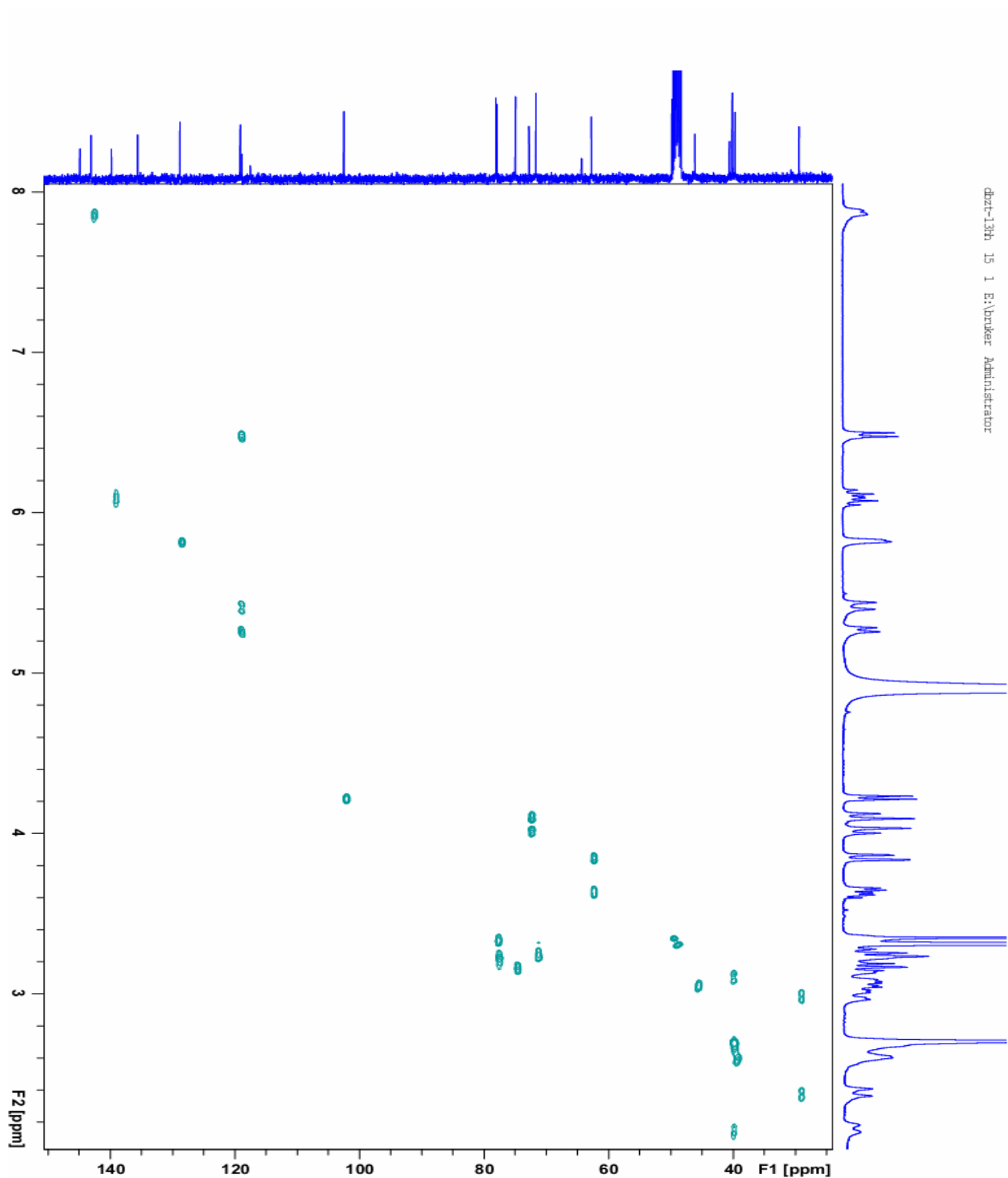
Figure S22. HSQC spectrum of compound 4.
