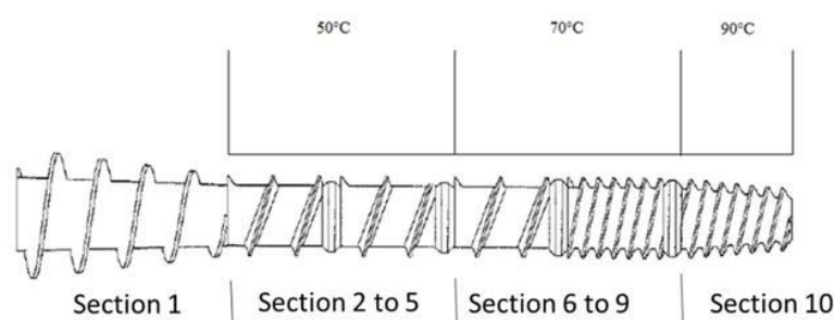
Figure 2. Extruder screw profile used to extrude the experimental diets control (CON), whole sorghum (WSD), flour (FLD) and mill-feed (MF).
