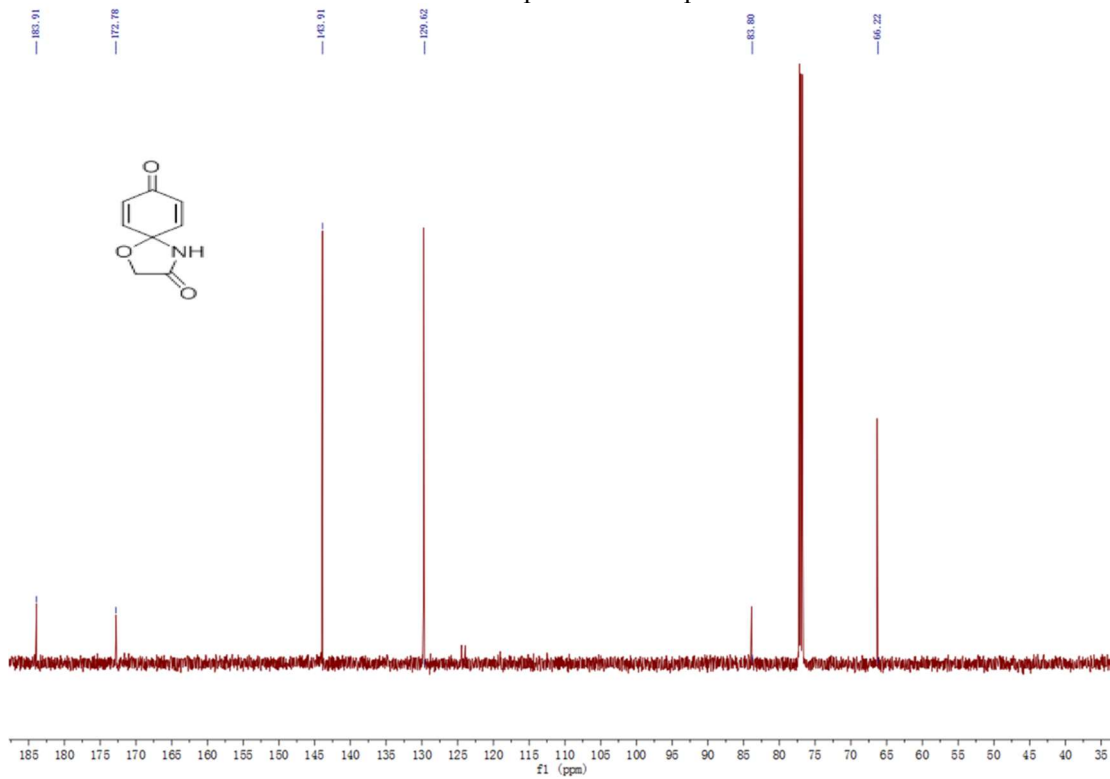
13 C NMR spectra of compound 10a
