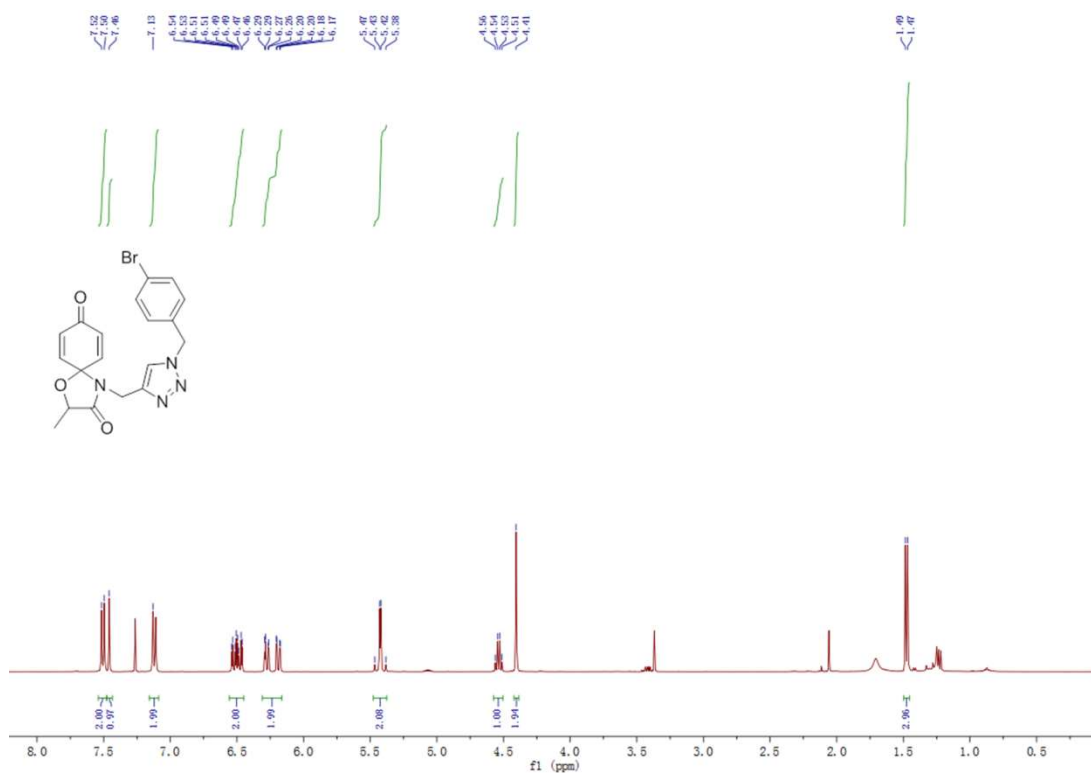
1 H NMR spectra of compound 12c
