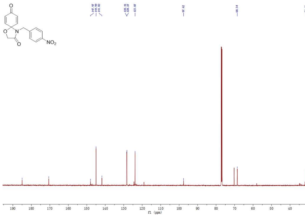
13 C NMR spectra of compounds 11i
