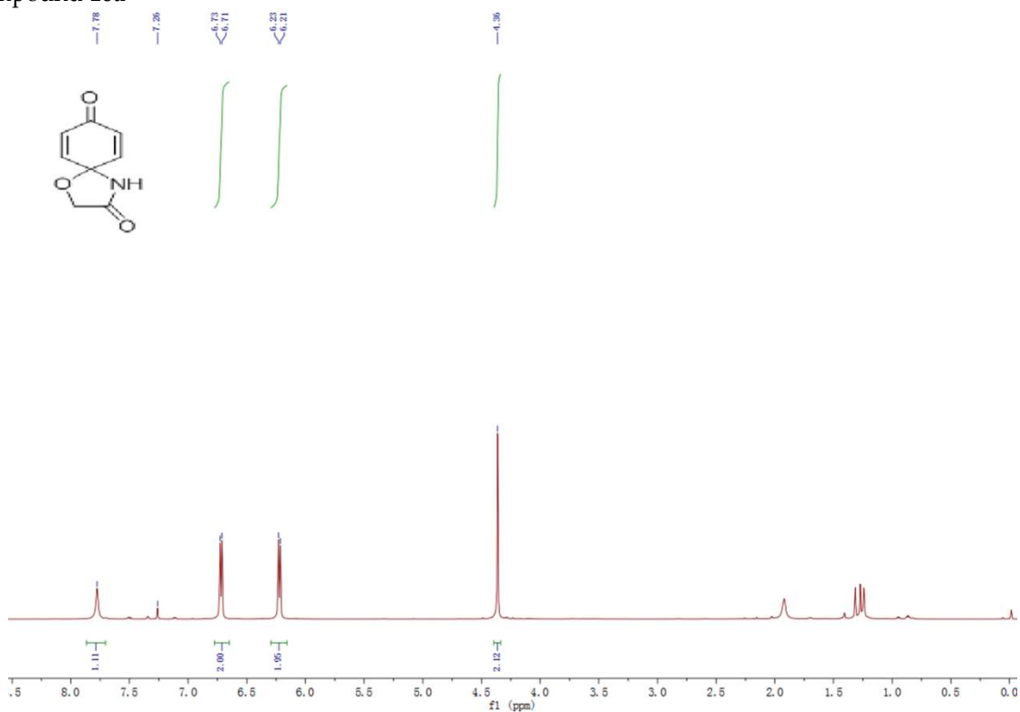
1 H NMR spectra of compound 10a
