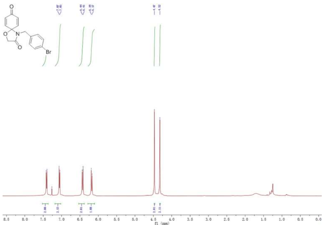
1 H NMR spectra of compound 11h
