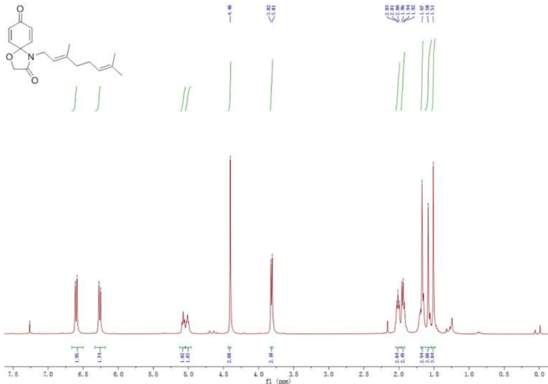
1 H NMR spectra of compound 11f
