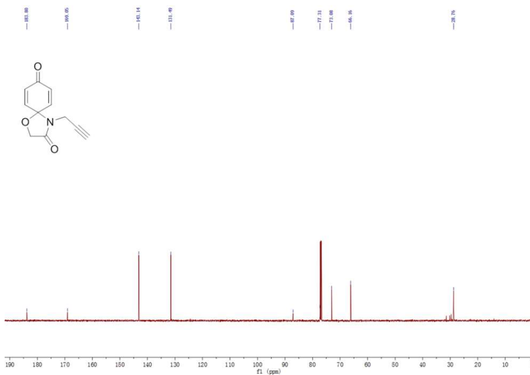
13 C NMR spectra of compounds 11c
