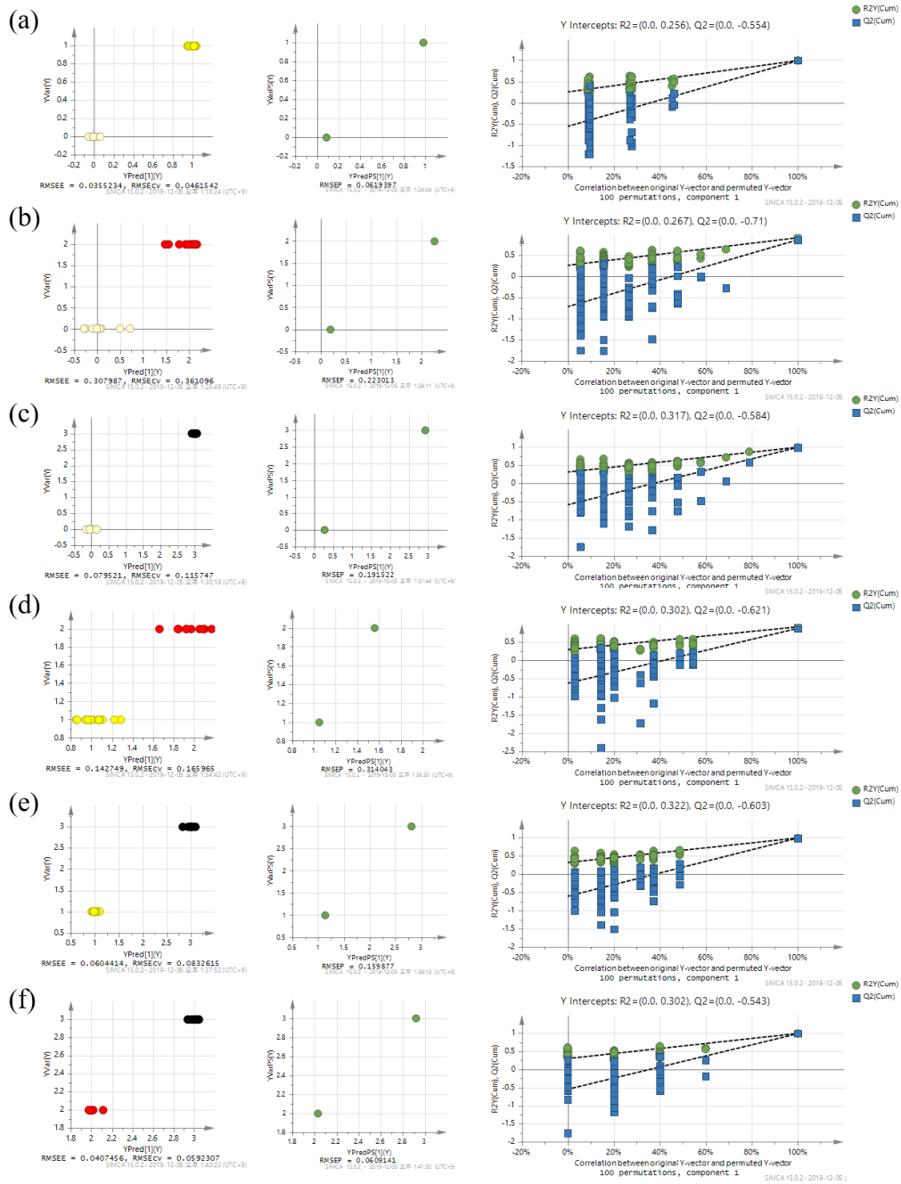
Figure 1. Results of OPLS model validation. (a) White ginseng vs. tae-geuk ginseng, (b) white ginseng vs. red ginseng, (c) white ginseng vs. black ginseng, (d) tae-geuk ginseng vs. red ginseng, (e) tae-geuk ginseng vs. black ginseng, (f) red ginseng vs. black ginseng.
