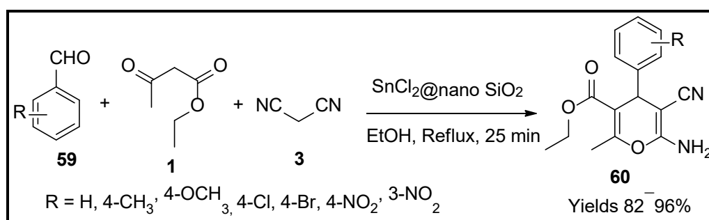
Scheme 20. Pyran derivatives synthesised by \text{SnCl}_2@\text{nano SiO}_2 catalyst.
