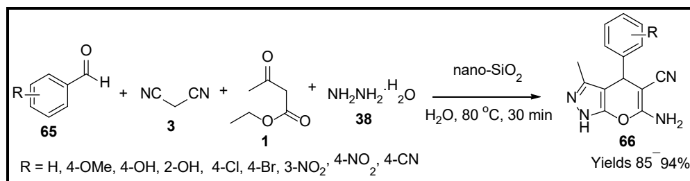
Scheme 23. Pyran derivatives synthesised by nano-SiO 2 catalyst.
