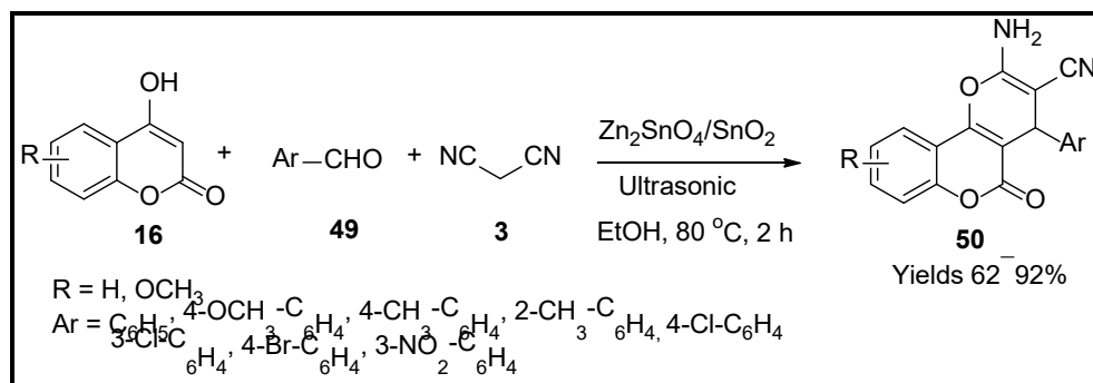
Scheme 16. Pyran derivatives synthesised by \text{Zn}_2\text{SnO}_4/\text{SnO}_2 catalyst.
