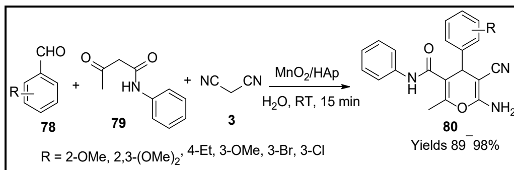
Scheme 28. Pyran derivatives synthesised by MnO 2 /HAp catalyst.
