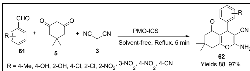
Scheme 21. Pyran derivatives synthesised by organosilica nanocatalyst.
