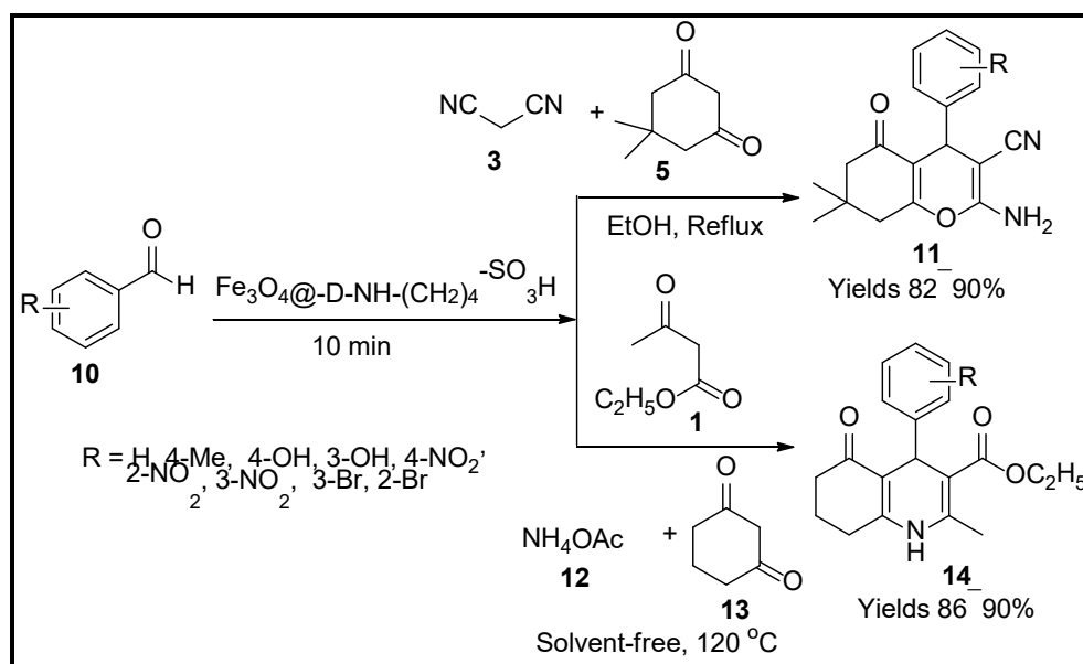
Scheme 4. Pyran derivatives synthesised by \text{Fe}_3\text{O}_4@-\text{D-NH}-(\text{CH}_2)_4-\text{SO}_3\text{H} catalyst.
