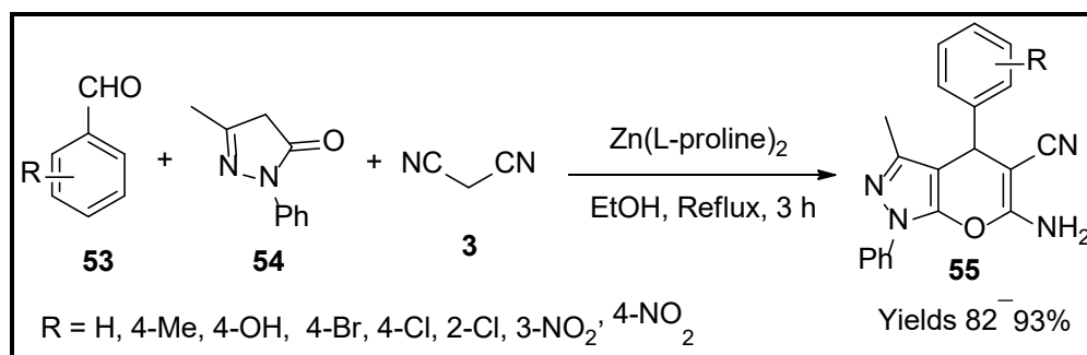
Scheme 18. Pyran derivatives synthesised by \text{Zn}(\text{Proline})_2 catalyst.
