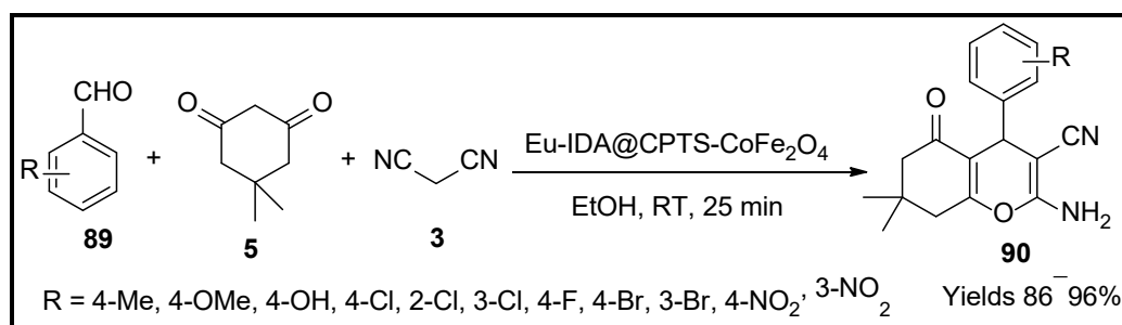
Scheme 31. Pyran derivatives synthesised by Eu-IDA@CPTS- \text{CoFe}_2\text{O}_4 catalyst.
