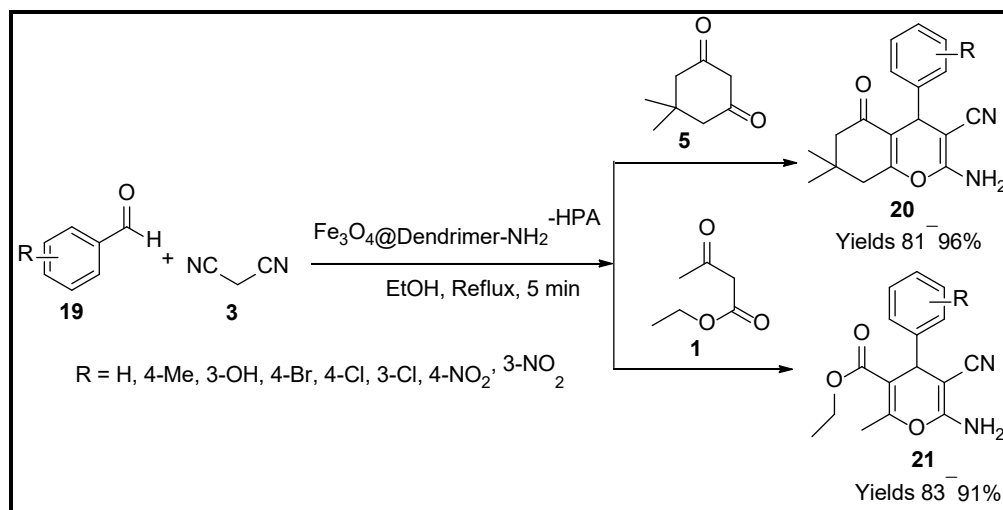
Scheme 6. Pyran derivatives synthesised by \text{Fe}_3\text{O}_4\text{@Dendrimer-NH}_2\text{-HPA} catalyst.
