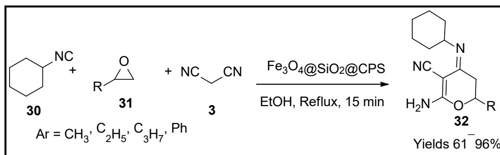
Scheme 10. Pyran derivatives synthesised by \text{Fe}_3\text{O}_4/\text{SiO}_2/\text{CPS} catalyst.
