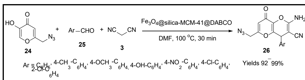
Scheme 8. Pyran derivatives synthesised by \text{Fe}_3\text{O}_4\text{@silica-MCM-41@DABCO} catalyst.
