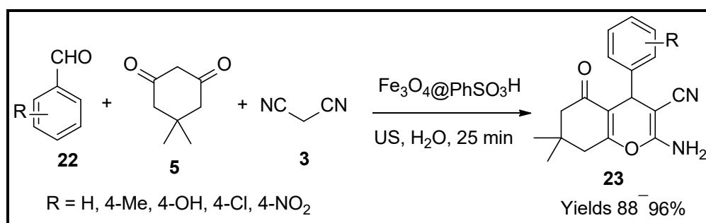
Scheme 7. Pyran derivatives synthesised by \text{Fe}_3\text{O}_4\text{@PhSO}_3\text{H} catalyst.
