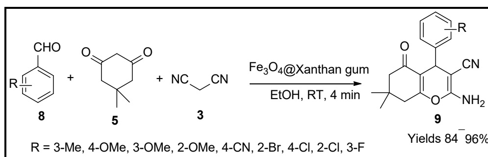
Scheme 3. Pyran derivatives synthesised by \text{Fe}_3\text{O}_4@\text{Xanthan gum} catalyst.
