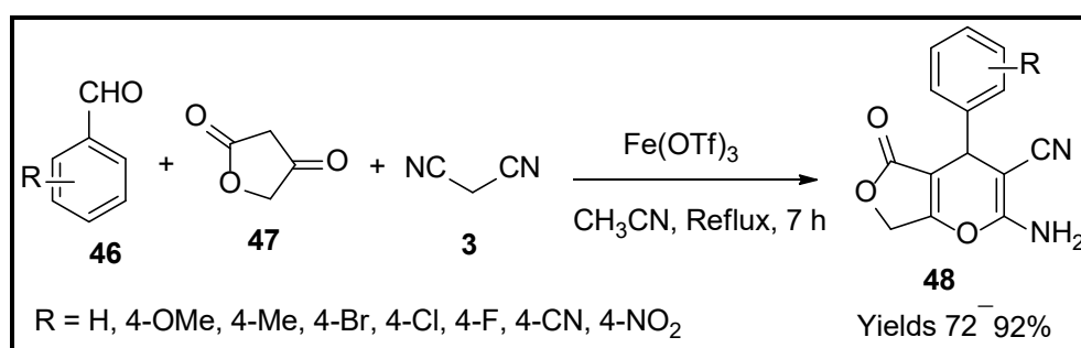
Scheme 15. Pyran derivatives synthesised by \text{Fe}(\text{OTf})_3 catalyst.
