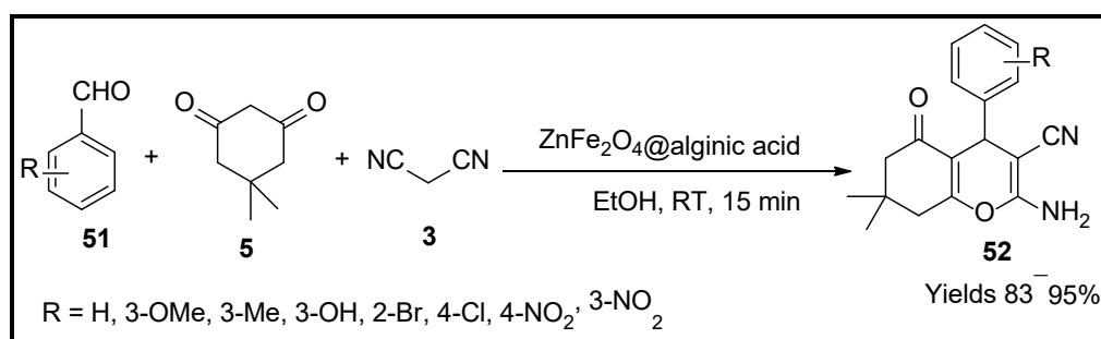
Scheme 17. Pyran derivatives synthesised by \text{ZnFe}_2\text{O}_4 catalyst.
