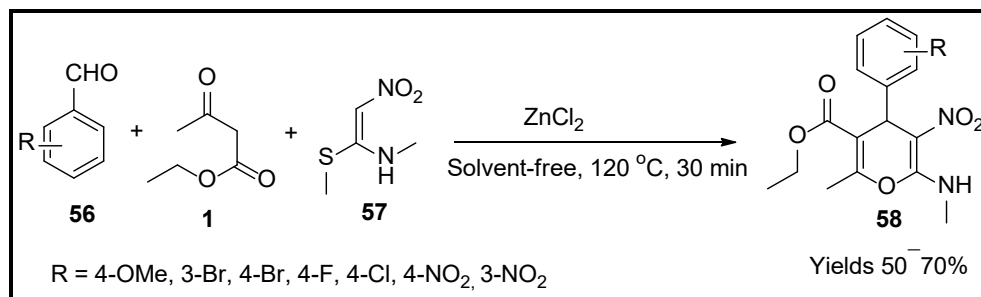
Scheme 19. Pyran derivatives synthesised by \text{ZnCl}_2 catalyst.
