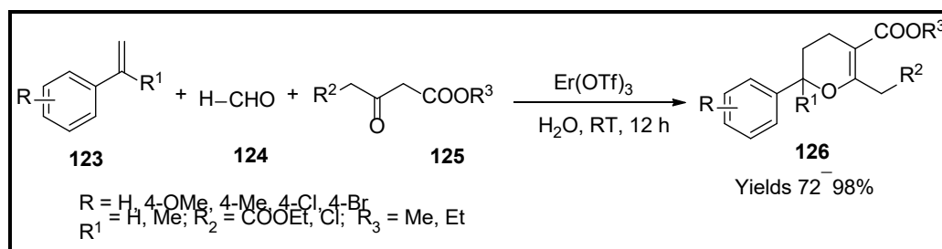
Scheme 43. Dihydropyran derivatives synthesised by \text{Er}(\text{OTf})_3 catalyst.
