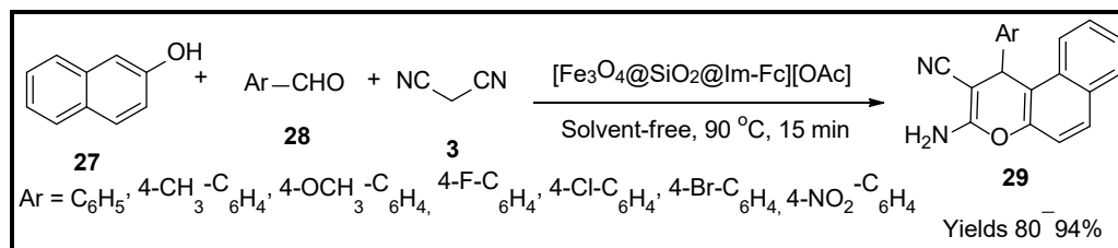
Scheme 9. Pyran derivatives synthesised by [\text{Fe}_3\text{O}_4/\text{SiO}_2/\text{Im-Fc}][\text{OAc}] catalyst.
