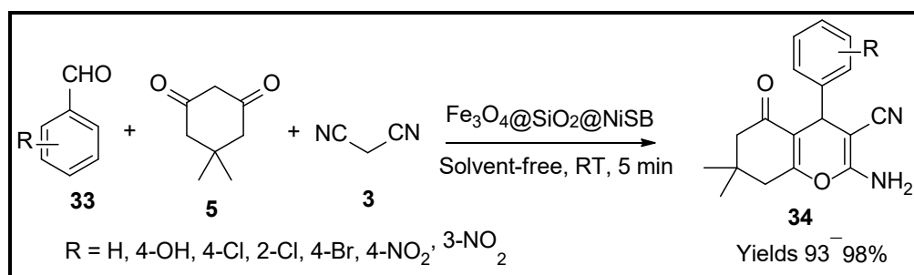
Scheme 11. Pyran derivatives synthesised by \text{Fe}_3\text{O}_4@\text{SiO}_2@\text{NiSB} catalyst.
