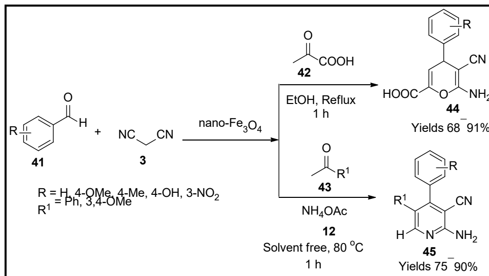
Scheme 14. Pyran derivatives synthesised by nano- \text{Fe}_3\text{O}_4 catalyst.
