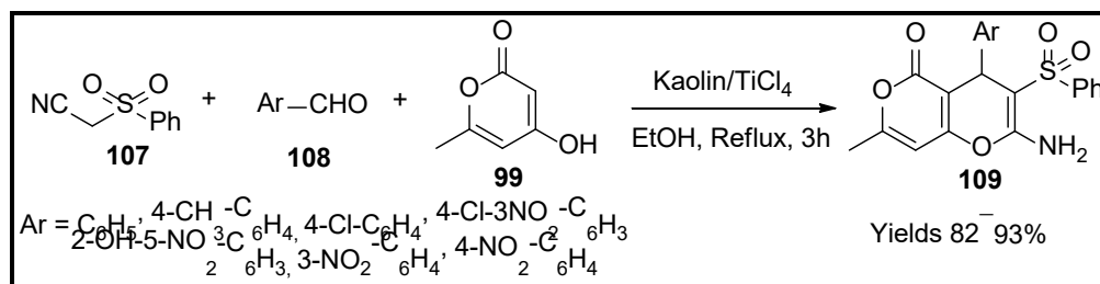
Scheme 38. Pyran derivatives synthesised by Kaolin/TiCl 4 nanocatalyst.
