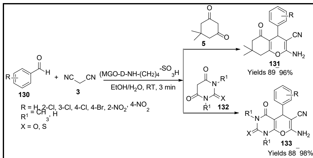
Scheme 45. Pyran derivatives synthesised by MGO-D-NH-(CH 2 ) 4 -SO 3 H catalyst.
