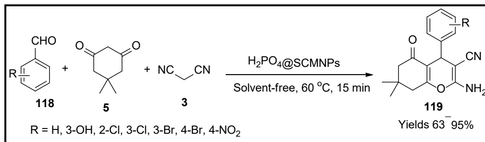
Scheme 41. Pyran derivatives synthesised by H 2 PO 4 @SCMNPs catalyst.
