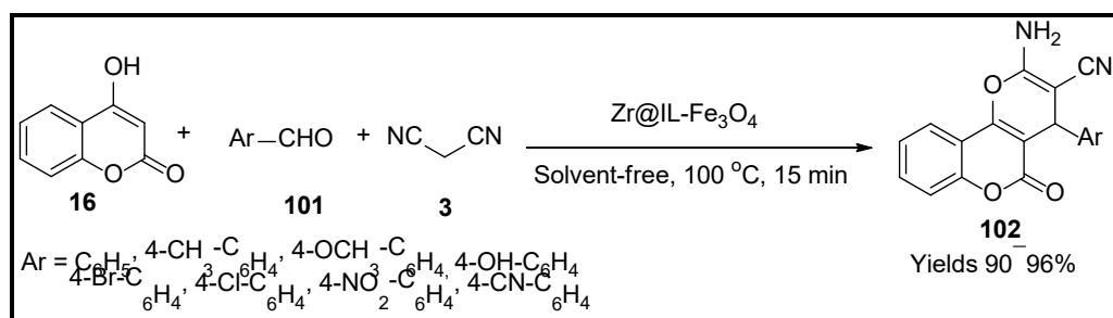
Scheme 36. Pyran derivatives synthesised by \text{Zr@IL-Fe}_3\text{O}_4 catalyst.
