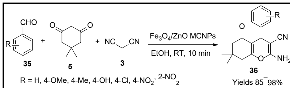
Scheme 12. Pyran derivatives synthesised by \text{Fe}_3\text{O}_4/\text{ZnO} MCNPs catalyst.
