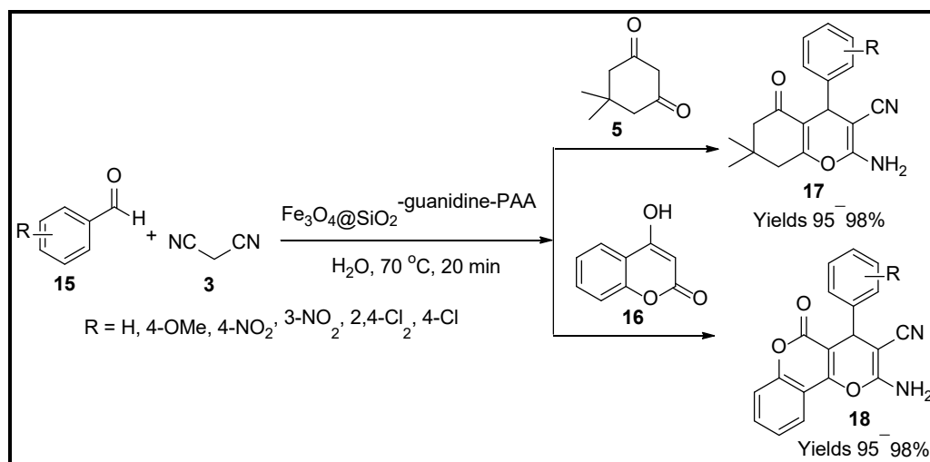
Scheme 5. Pyran derivatives synthesised by \text{Fe}_3\text{O}_4@-\text{SiO}_2\text{-guanidine-PAA} catalyst.
