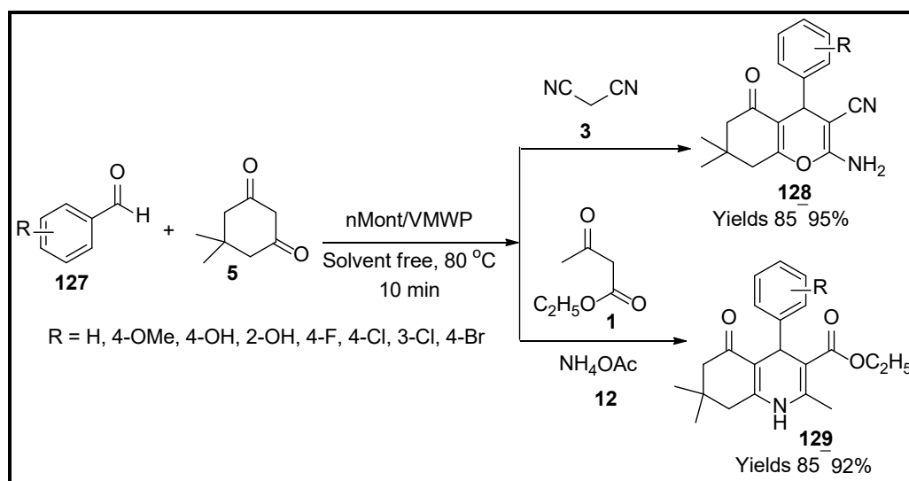
Scheme 44. Pyran derivatives synthesised by n Mont/VMWP catalyst.
