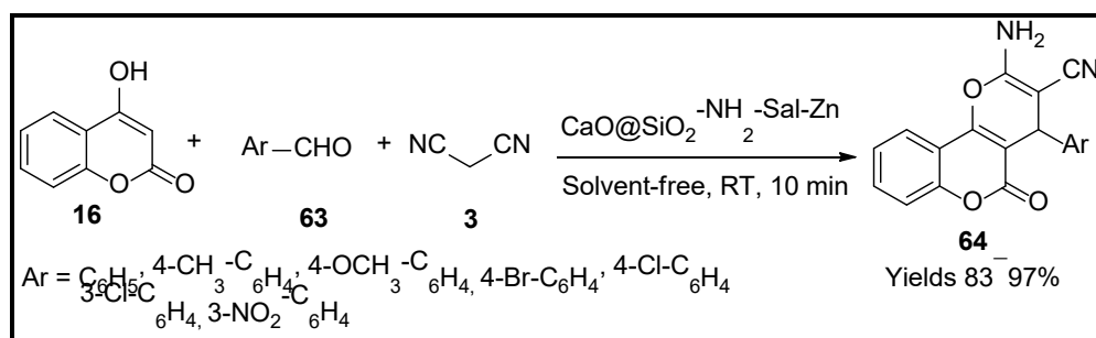
Scheme 22. Pyran derivatives synthesised by CaO@SiO 2 -NH 2 -Sal-Zn catalyst.
