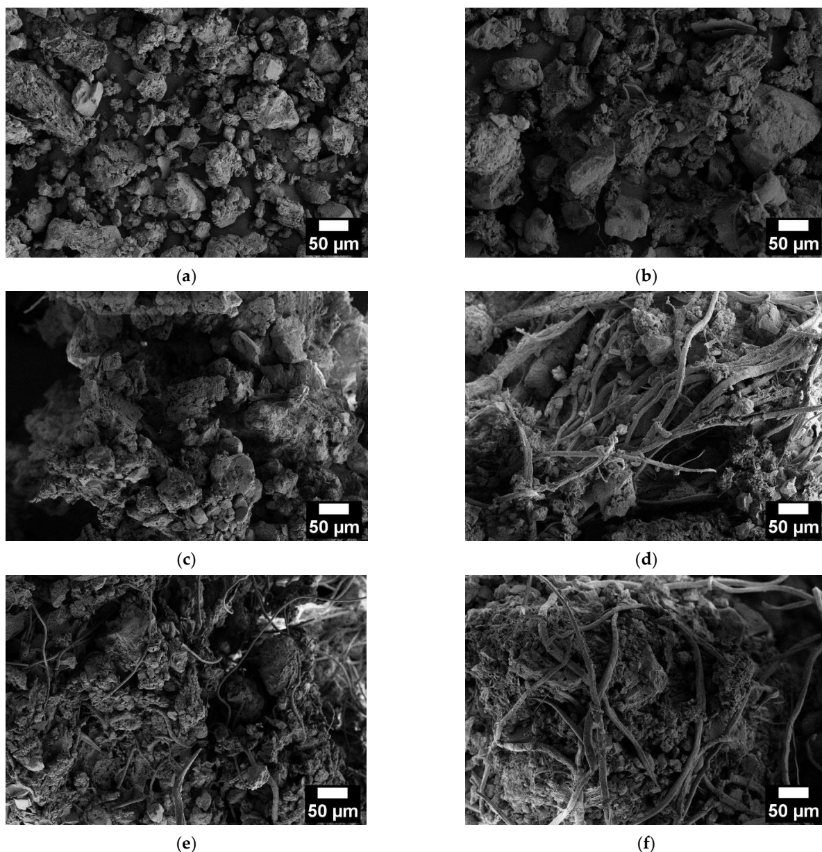
Figure 6. SEM micrographs of the (a) neat soil and soil mixed with (b) X1, (c) X1W2, (d) X1W5, (e) X4W2, and (f) X4W5 hydrogels.
