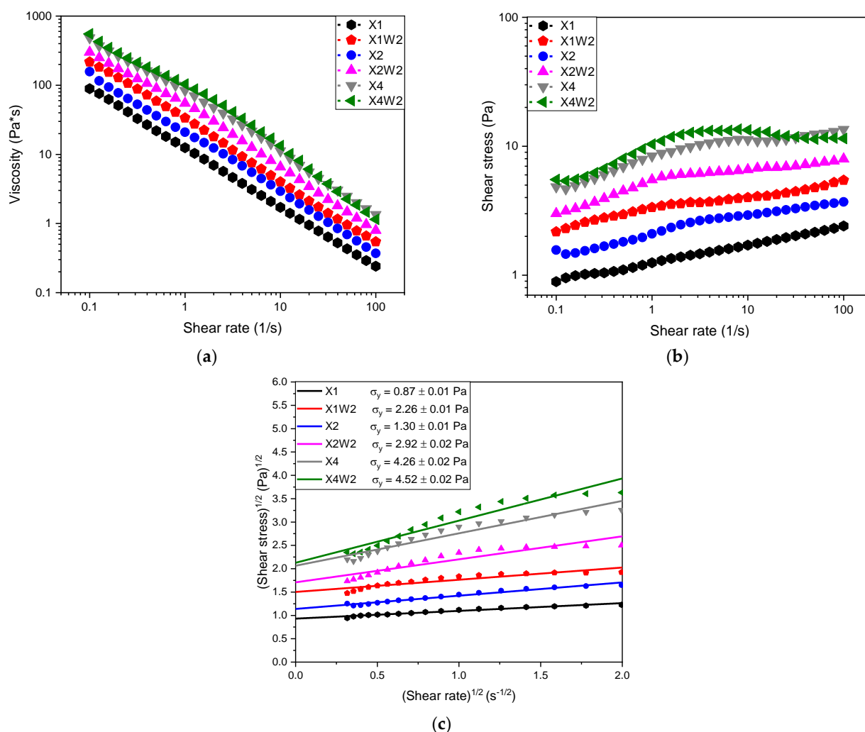
Figure 1. Rheological tests on the hydrogel composites. Trends of (a) shear viscosity and (b) shear stress as a function of the shear rate. (c) Linear interpolation of shear stress values for the determination of the yield stress, according to the Casson model (see Equation (1)).
