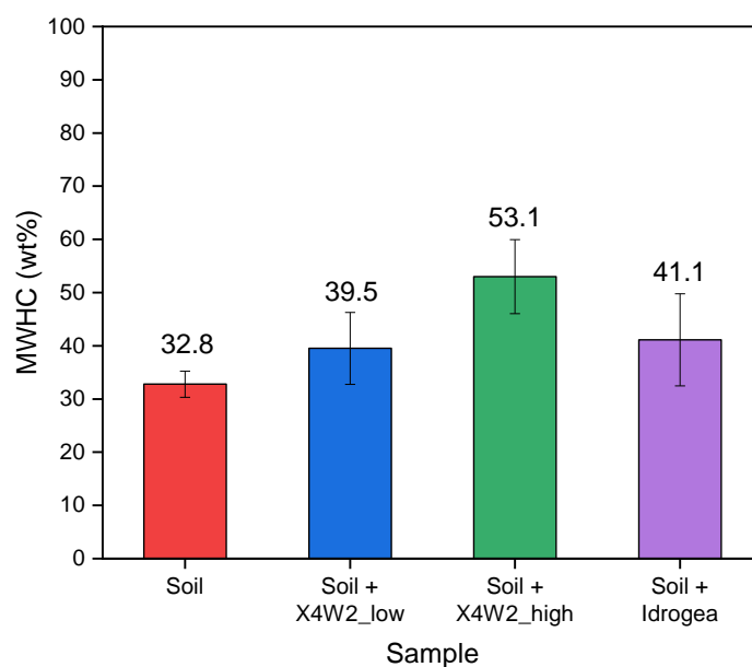
Figure 7. Maximum water holding capacity of soil with X4W2 samples ( low and high ) and Idrogea.
