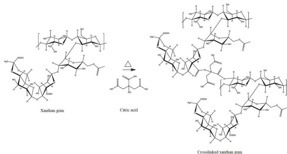
Figure 14. Reaction scheme of the xanthan gum with citric acid (reprinted with permission from [67]).
