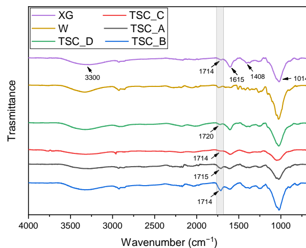
Figure 2. FT-IR analysis on the TSC composites and neat materials.
