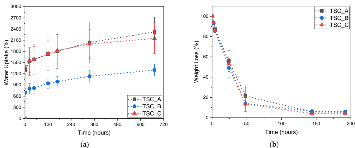
Figure 5. Evaluation of the (a) water uptake and of the (b) weight loss for the prepared xanthan gum-based TSC.
