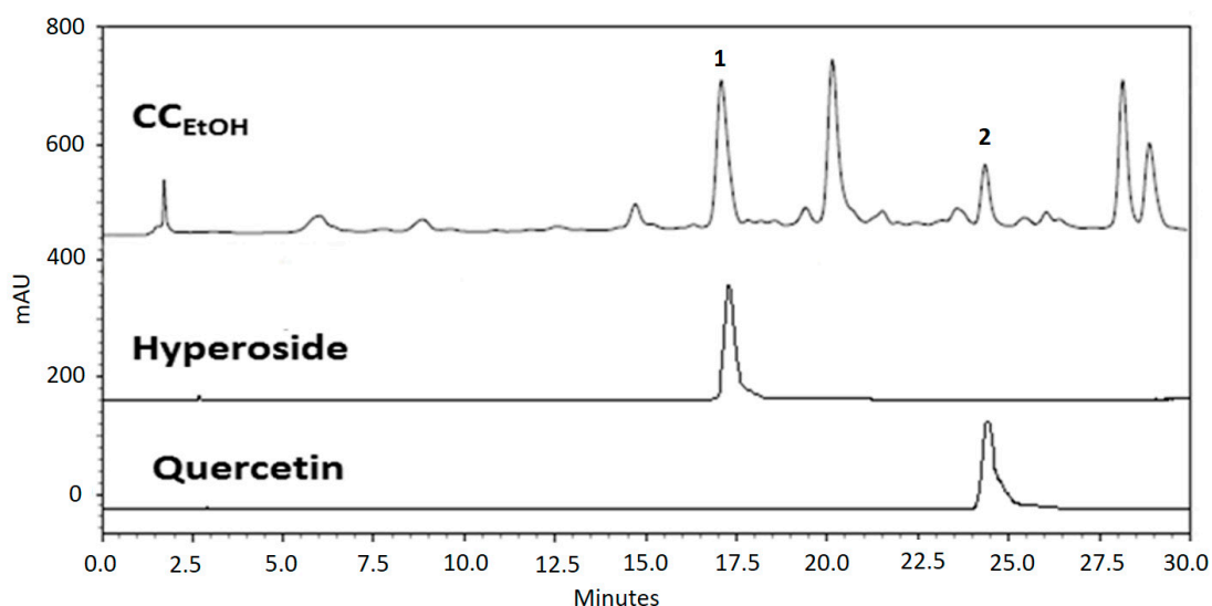
Figure S1. HPLC chromatographs of the ethanol extract of Cuscuta campestris whole plant and standards (hyperoside and quercetin). Peaks 1 and 2 are hyperoside and quercetin, respectively.
