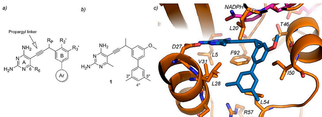
Figure 10. Propargyl-linked antifolates. a) General scaffold with the diaminopyrimidine ring (A), phenyl ring (B) and aryl ring (Ar) along with possible positions for substitutions (R6, RP, R29 and R39). b) A concrete example of a propargyl-linked antifolate, a biphenyl one, with labeled atom positions (compound 1). c) Active site of a resistant DHFR, showing active site residues (orange), NADPH (magenta) and compound 1 (blue). Reproduced from Viswanathan et al [120].
