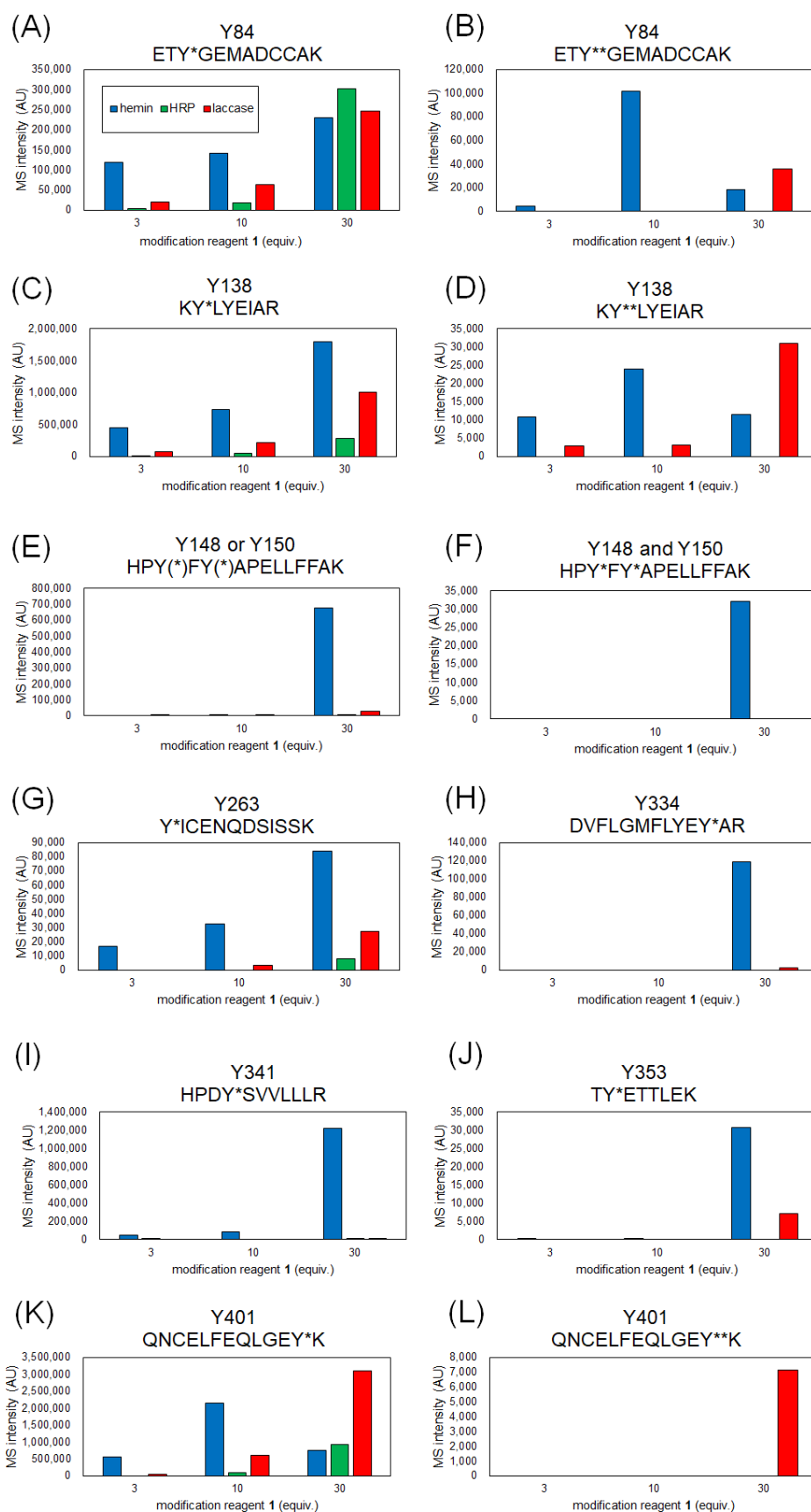
Figure 3. MS intensity comparison of modified peptides containing each tyrosine residue. Y* and Y** indicate single and double modified tyrosines with 1. Peptide fragment containing modified
