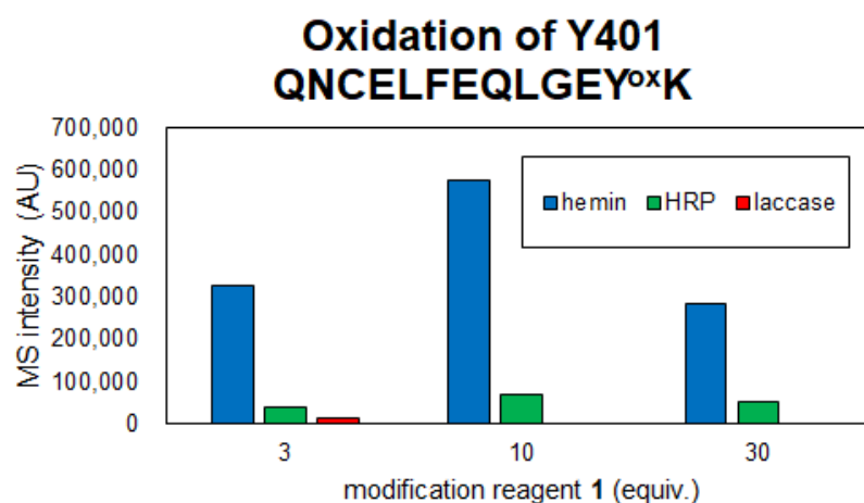
Figure 4. Detection of oxidized peptide of Y401 in each reaction condition.
