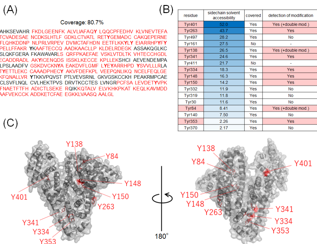
Figure 2. Tyrosine residues in modified HSA. (A) Amino acid sequences of HSA and peptide fragments detected by nanoLC-MS/MS analysis. (B) Sidechain solvent accessibility of tyrosine residues and labeling sites. The peptide fragment containing Tyr161 and Tyr411 were not detected. (C) Mapping of modified tyrosine residues on 3D structures (PDB:1BM0).
