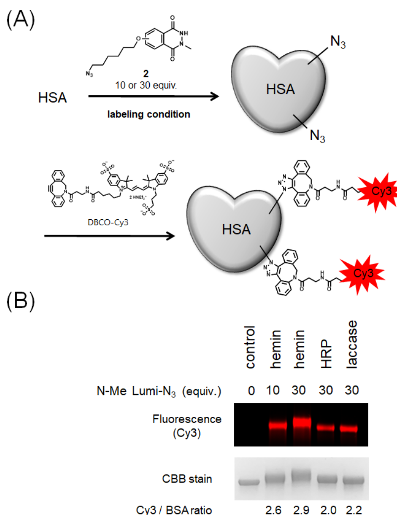
Figure 5. Modification of HSA with azide-conjugated N -methylated luminol derivative ( 2 ) and comparison of modification efficiencies. (A) Scheme of HSA modification using 2 and DBCO-Cy3. (B) Comparison of modification efficiency from Cy3 fluorescence intensity. N = 2. Representative fluorescent gel is shown in Figure 5B.
