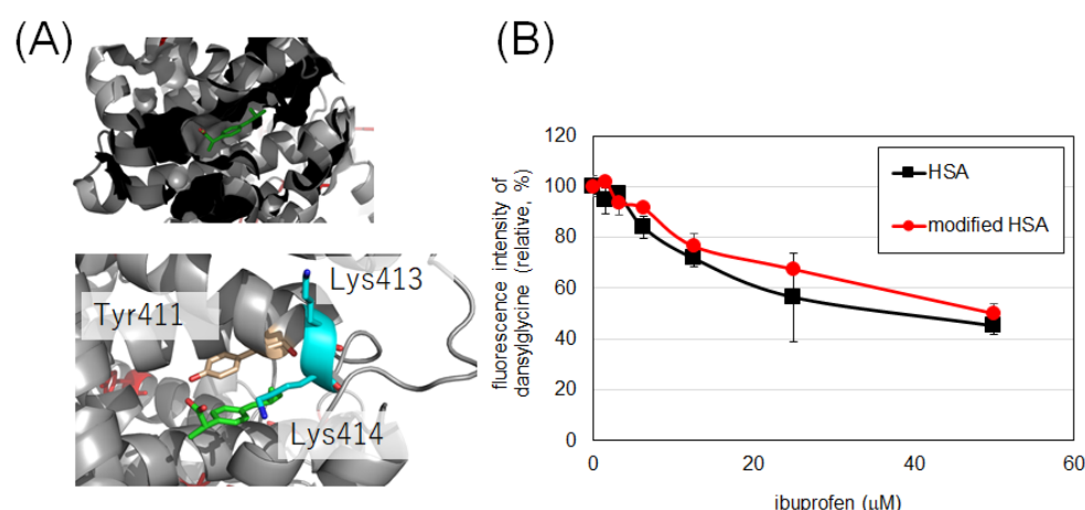
Figure 6. Binding of HSA and modified HSA to ibuprofen. (A) The binding of ibuprofen at Sudlow's site II (PDB: 6U4X). (B) Fluorescence changes due to competition between ibuprofen and dansylglycine. Error bars, mean \pm SD from three independent experiments. These experiments were performed at 25 °C (See Figure S16 for temperature-dependency).
