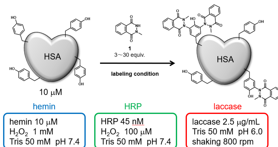
Figure 1. HSA modification by N -methylated luminol derivative (1) and three catalytic reaction conditions.
