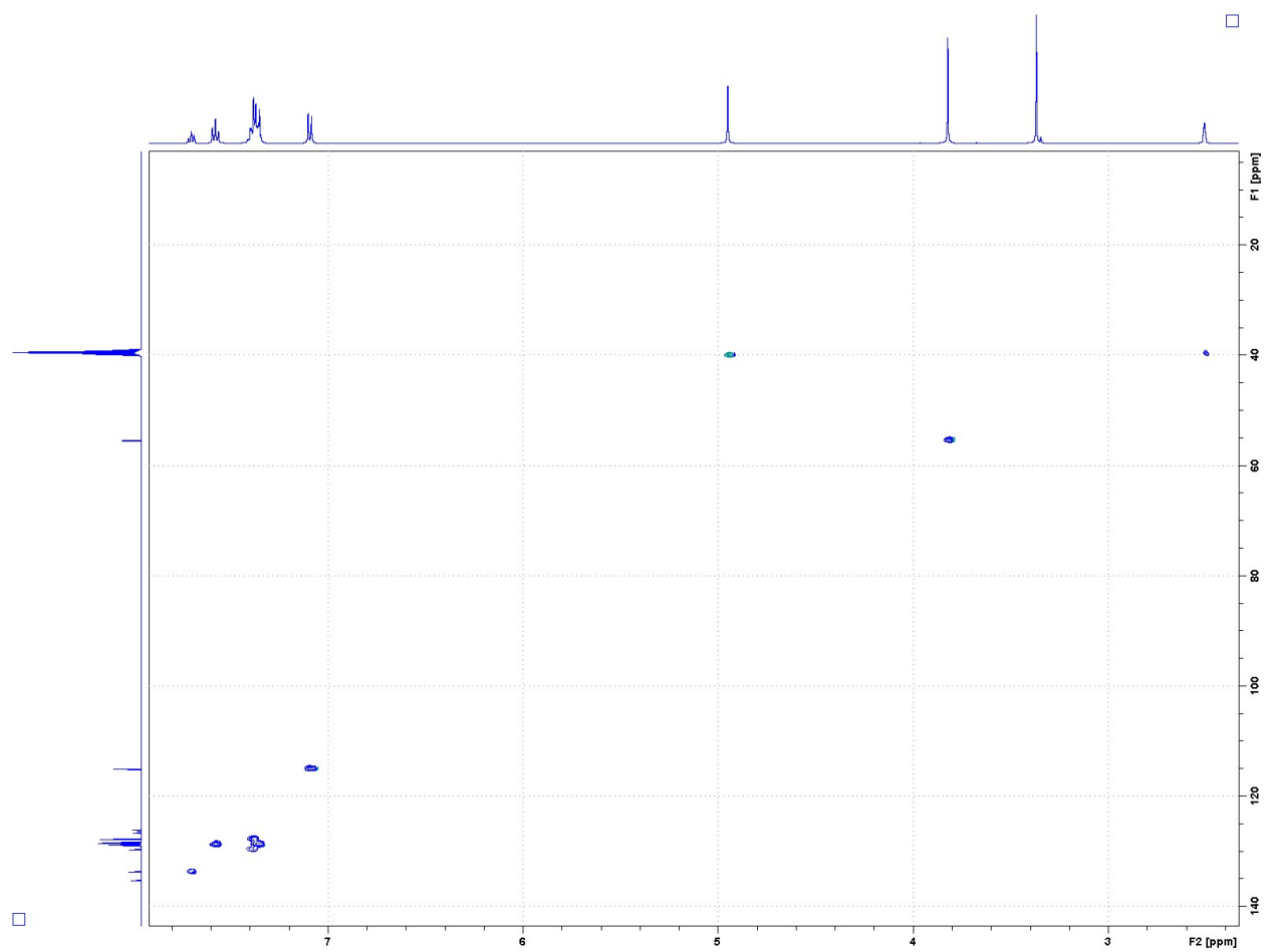
Figure S10. HSQCED ^1\text{H} - ^{13}\text{C} spectrum of compound 5 in \text{DMSO}-d_6 ;
