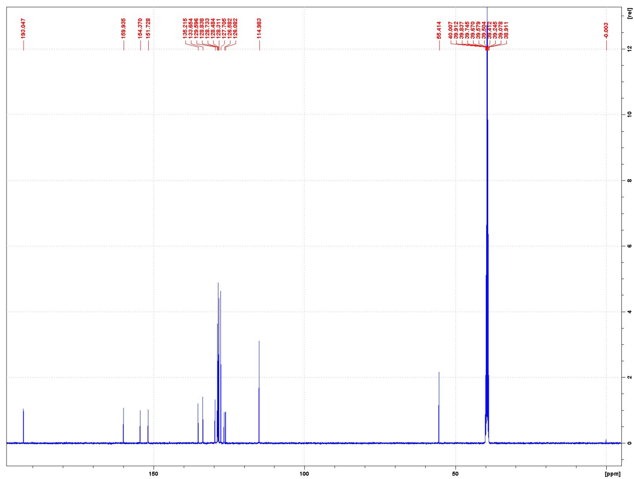
Figure S5. 13 C NMR spectrum of compound 5 in DMSO- d 6 ;
