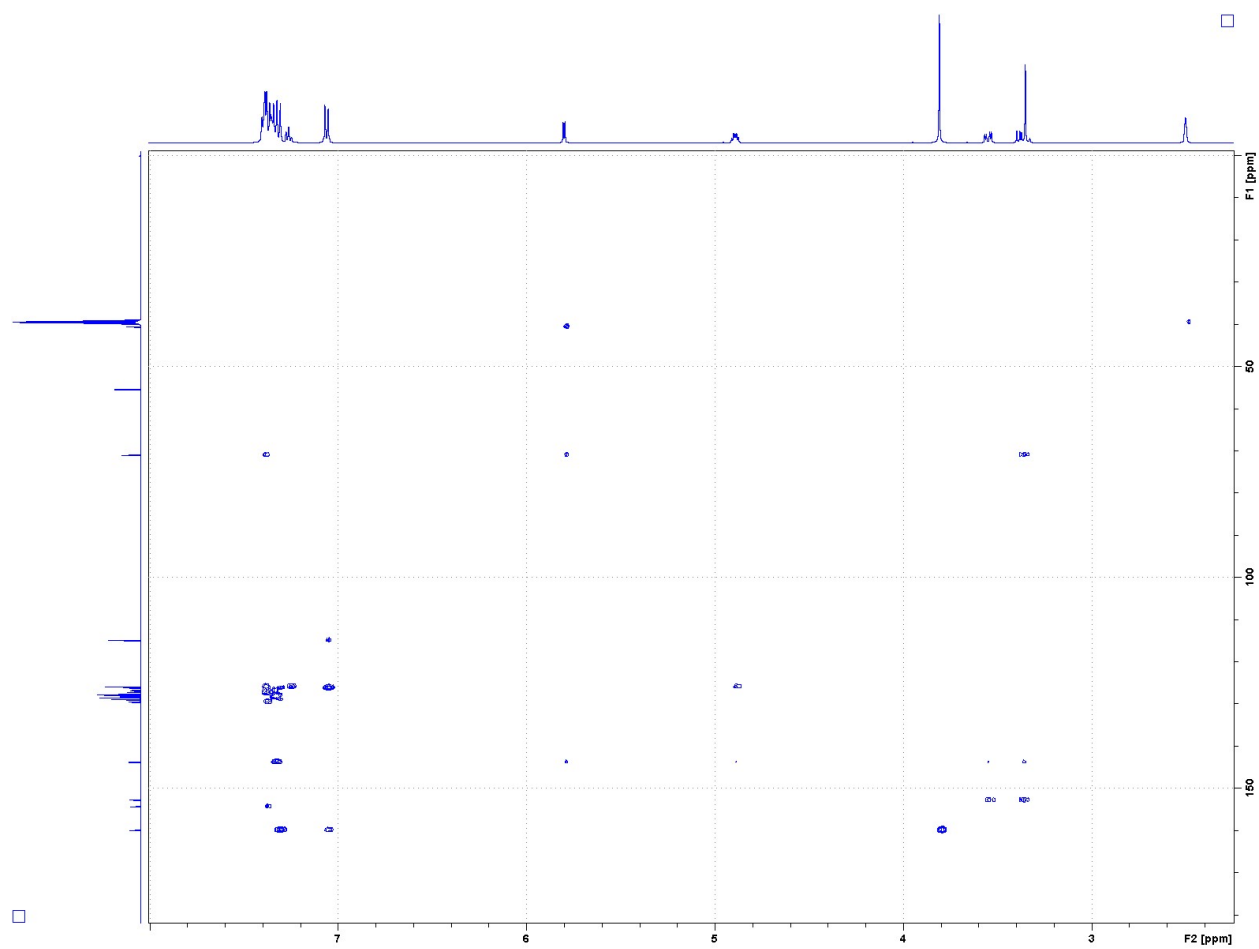
Figure S16. HMBC ^1\text{H} - ^{13}\text{C} spectrum of compound 6 in \text{DMSO}-d_6 ;
