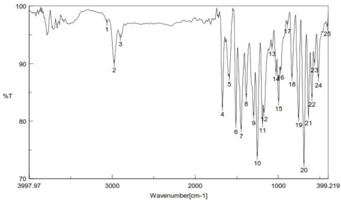
Figure S3. FT-IR spectrum of compound 5;
