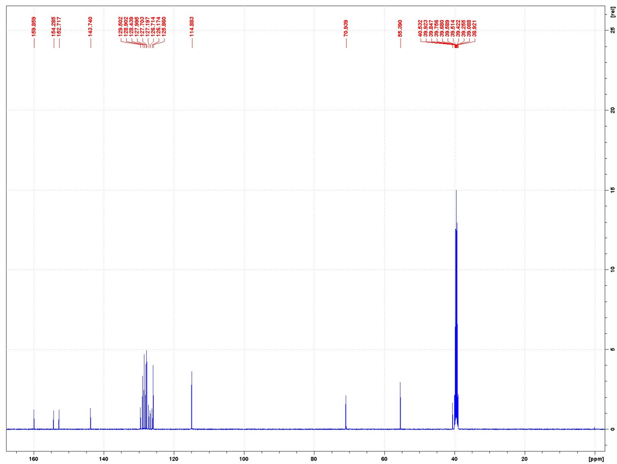
Figure S13. 13 C NMR spectrum of compound 6 in DMSO- d 6 ;
