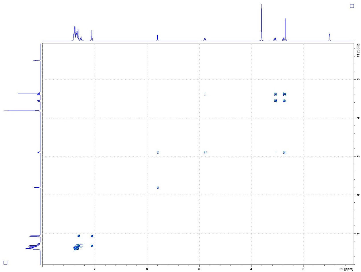
Figure S14. COSY ^1\text{H} - ^1\text{H} spectrum of compound 6 in \text{DMSO-}d_6 ;
