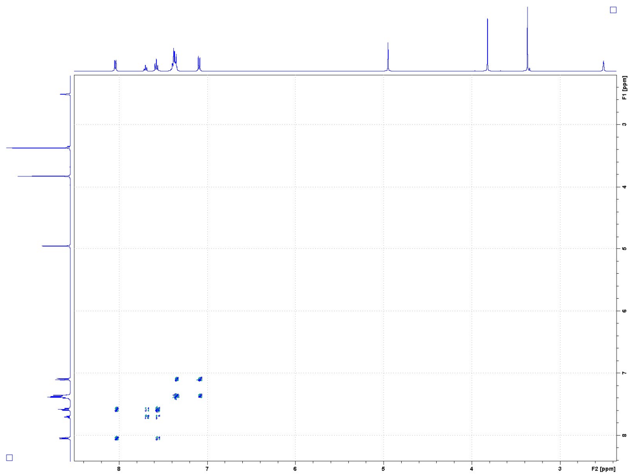
Figure S6. COSY ^1\text{H} - ^1\text{H} spectrum of compound 5 in \text{DMSO-}d_6 ;
