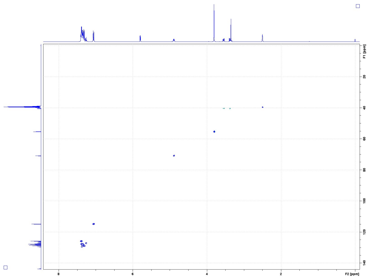
Figure S18. HSQCED ^1\text{H} - ^{13}\text{C} spectrum of compound 6 in \text{DMSO}-d_6 ;
