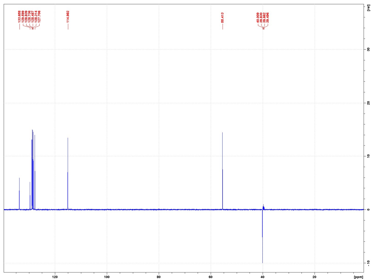
Figure S7. 13 C DEPT135 spectrum of compound 5 in DMSO- d 6 ;
