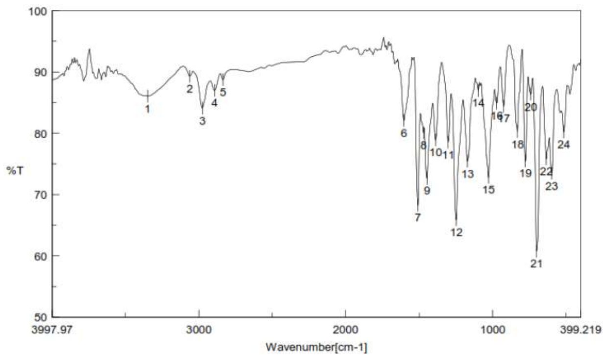
Figure S11. FT-IR spectrum of compound 6;
