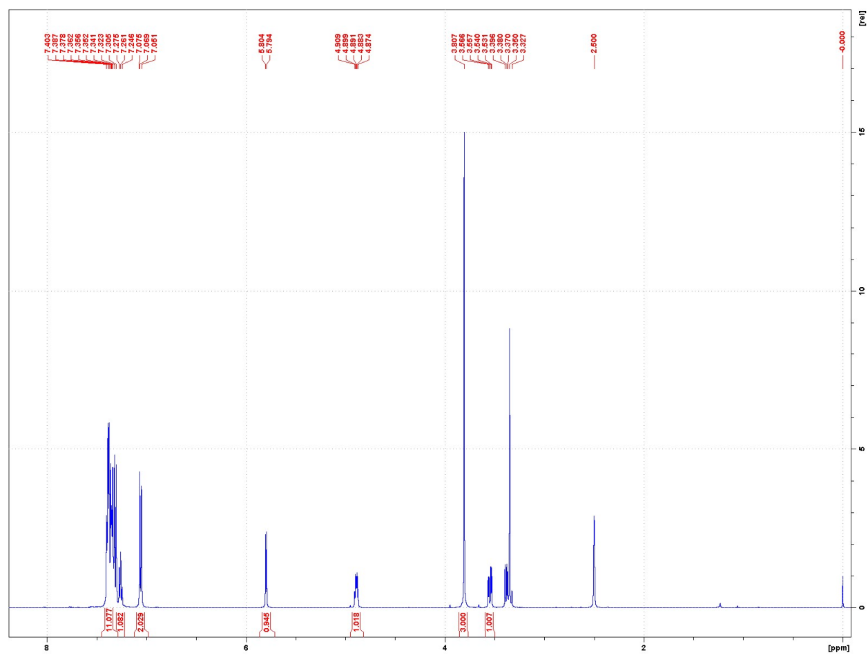
Figure S12. 1 H NMR spectrum of compound 6 in DMSO- d 6 ;
