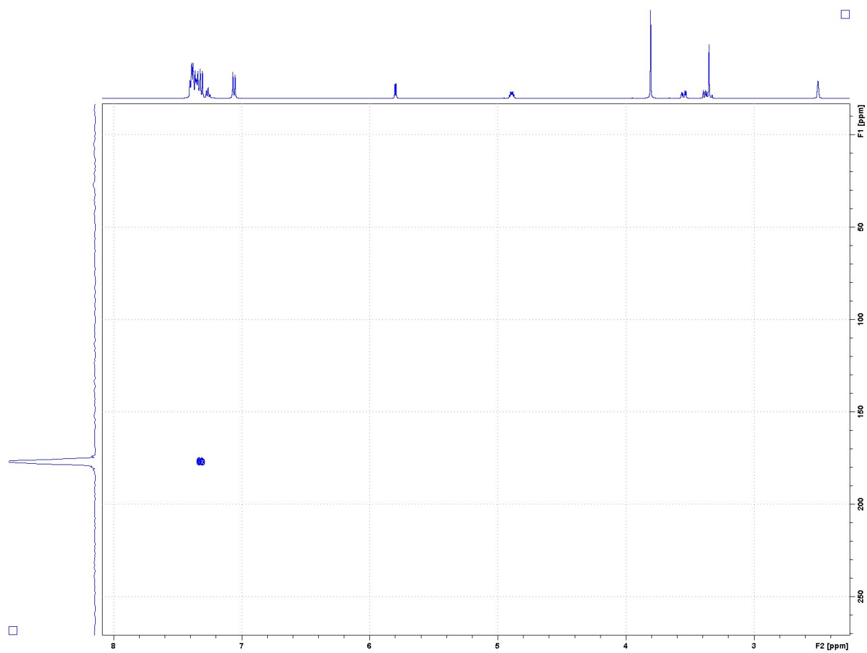
Figure S17. HMBC ^1\text{H} - ^{15}\text{N} spectrum of compound 6 in \text{DMSO-}d_6 ;
