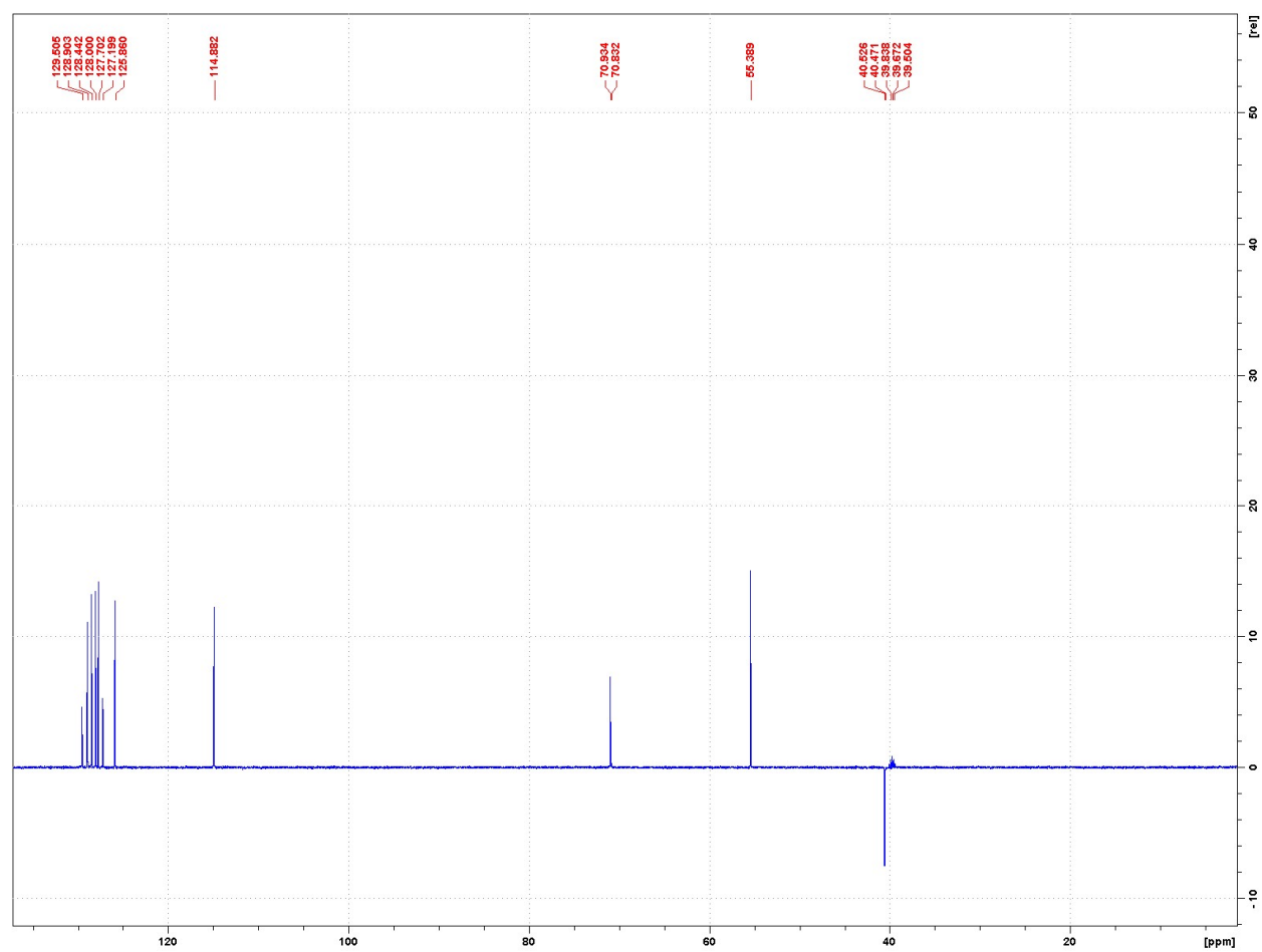
Figure 15. 13 C DEPT135 spectrum of compound 6 in DMSO- d 6 ;
