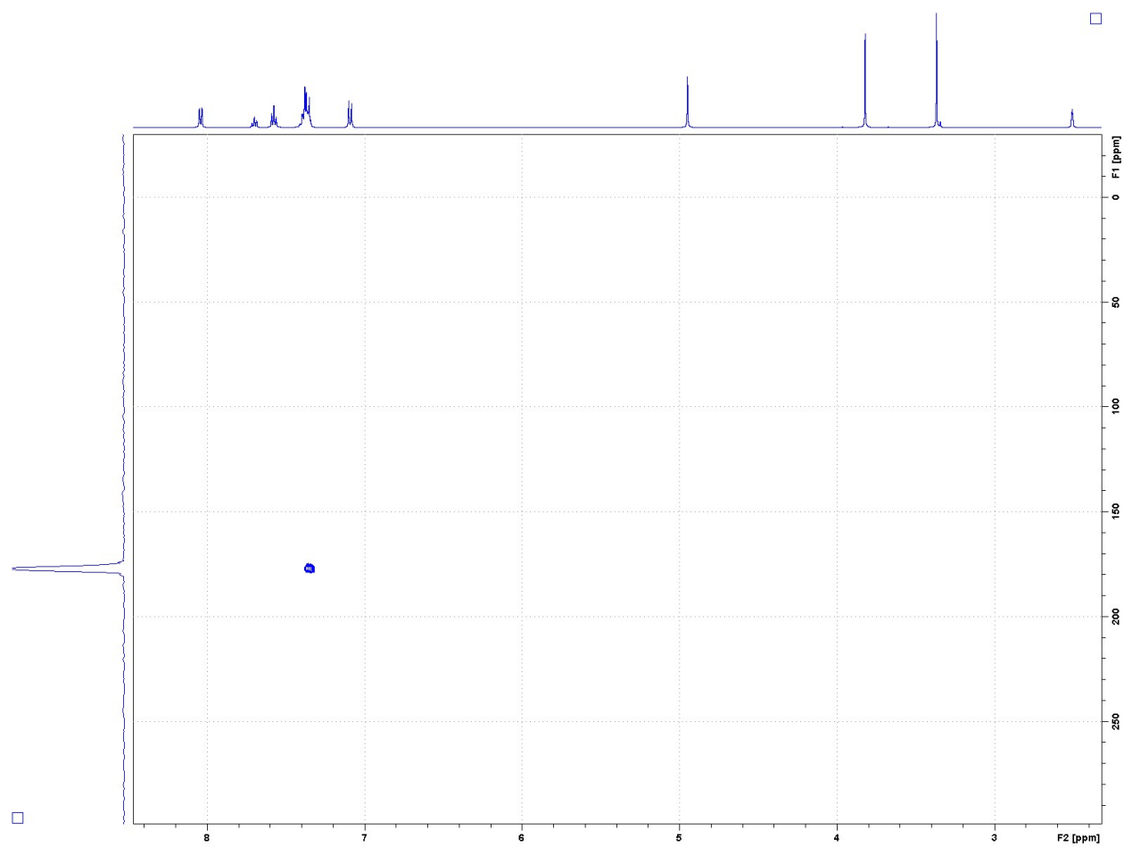
Figure S9. HMBC ^1\text{H} - ^{15}\text{N} spectrum of compound 5 in \text{DMSO}-d_6 ;
