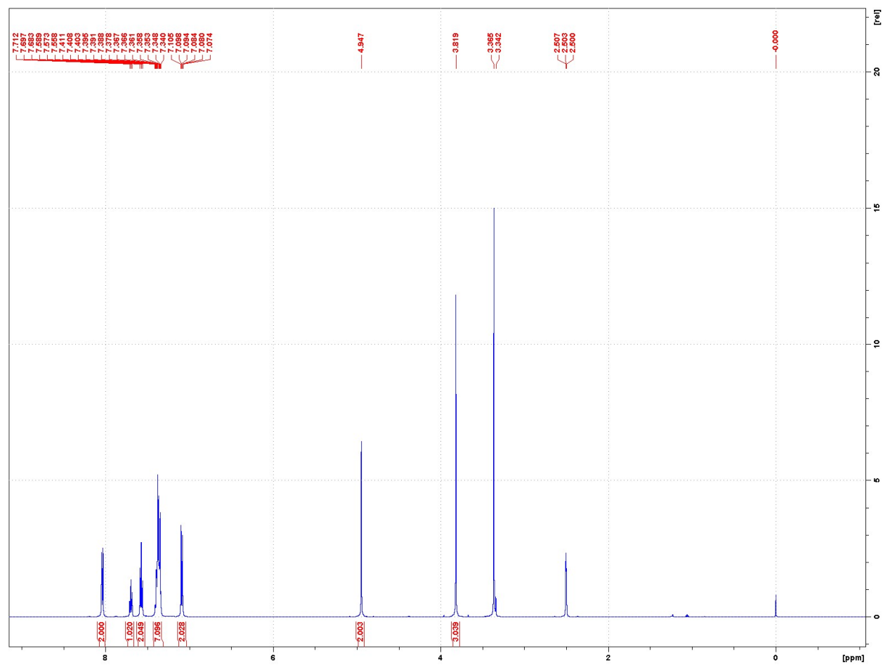
Figure S4. 1 H NMR spectrum of compound 5 in DMSO- d 6 ;
