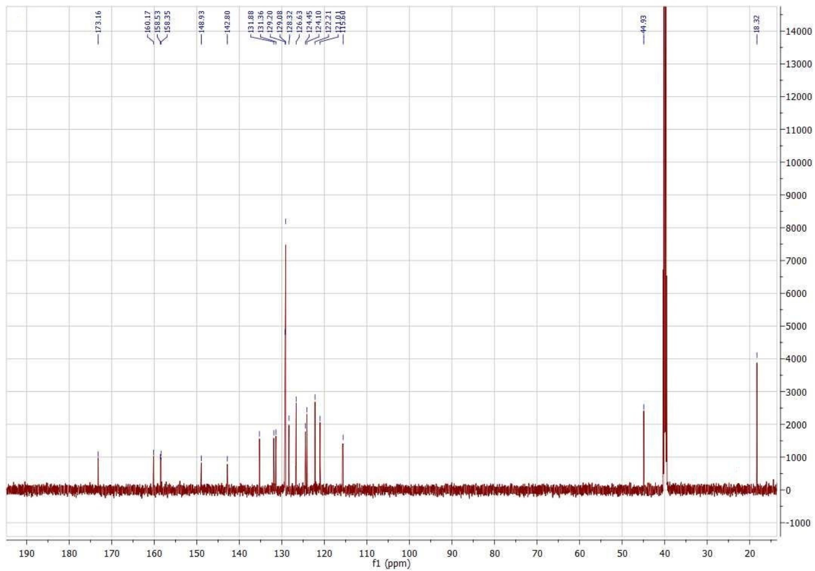
Figure S2. 13 C-NMR spectrum of compound 6.
