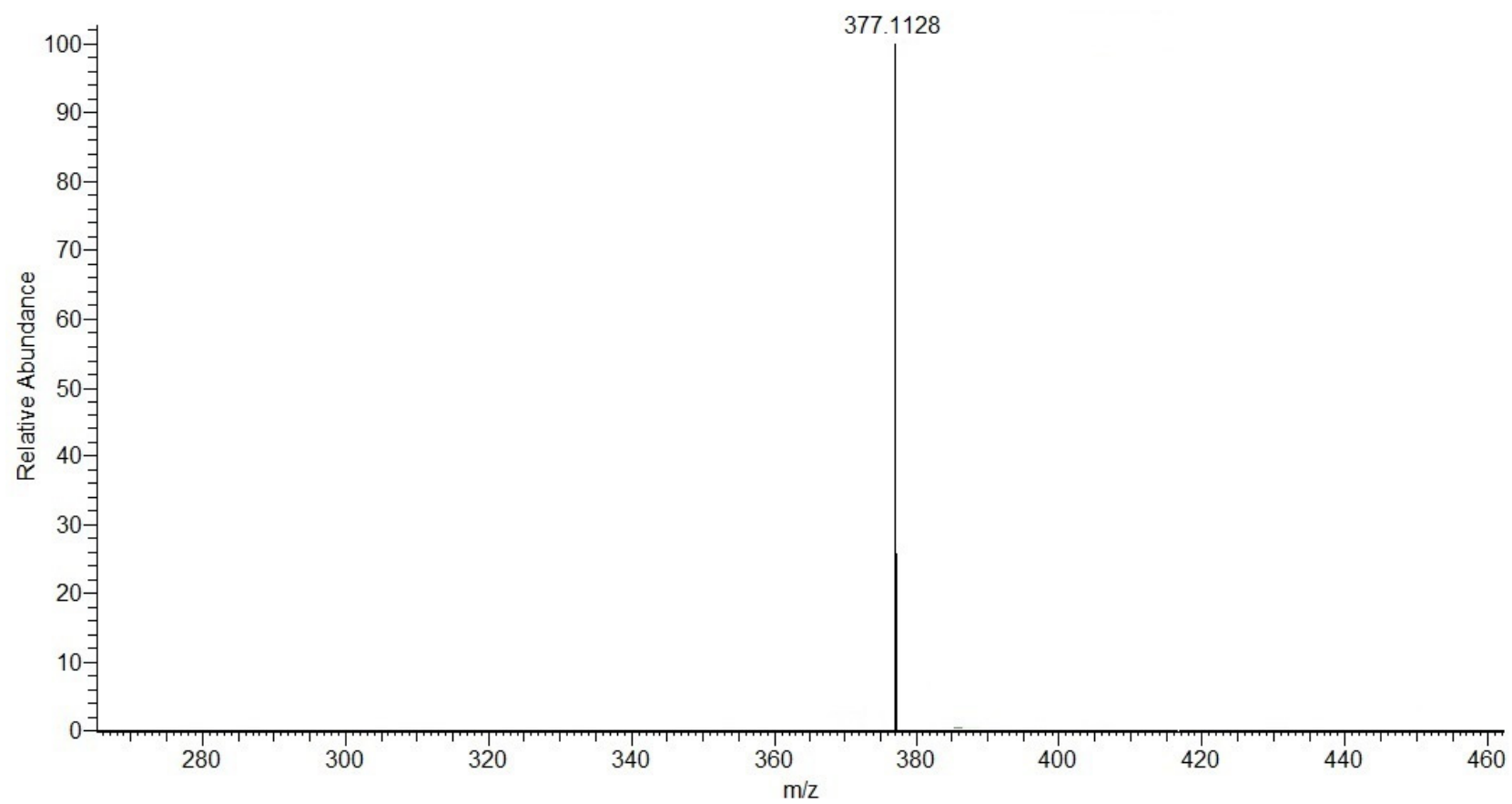
Figure S4. ESI-HRMS of compound 6 .
