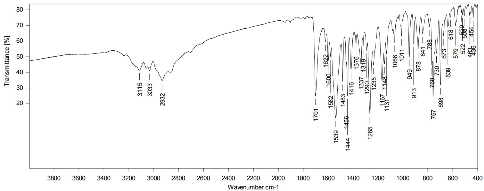
Figure S5. IR spectrum of compound 6 .
