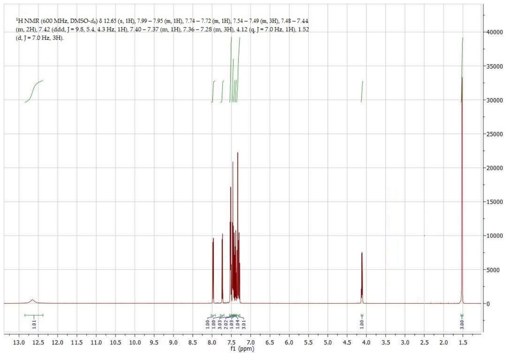
Figure S1. ^1\text{H} -NMR spectrum of compound 6 .
