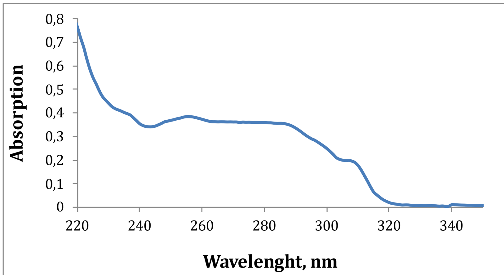
Figure S3. UV spectrum of compound 6.
