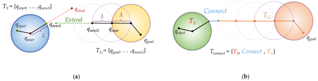
Figure 5. Process of RRT-connect algorithm: (a) extend from tree T_b with root as goal position q_{goal} to tree T_a with root as start position q_{start} ( T_a 's q_{near} extends in T_a 's q_{newS} direction); (b) as the paths P_a and P_b created in each tree are connected ("Connect") to each other, path P_{merged} is created.
