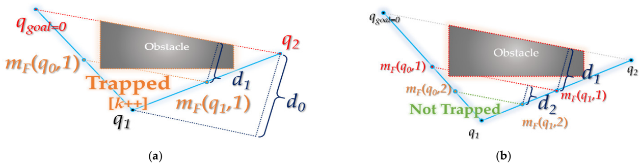
Figure 12. Details of forward interpolation process: (a) when the midpoint m_F(q_0,1) of the waypoints q_0, q_1 and the midpoint m_F(q_1,1) of q_1, q_2 are not collision-free from the obstacle; (b) when the midpoint m_F(q_0,2) of the midpoint m_F(q_0,1), q_1 and the midpoint m_F(q_1,2) of midpoint m_F(q_1,1), q_1 are not collision-free from the obstacle.
