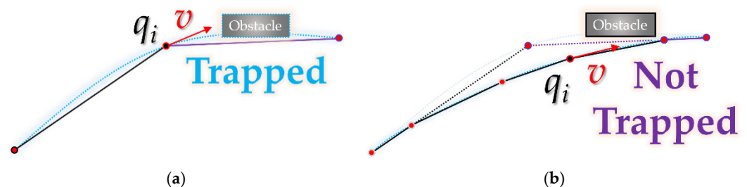
Figure 2. Path needing kinodynamic planning (when a mobile robot with kinematic constraints moves at a velocity v at an arbitral point q_i ): (a) situation in which the robot collides with the obstacle; (b) situation in which the obstacle is avoided by increasing waypoints.
