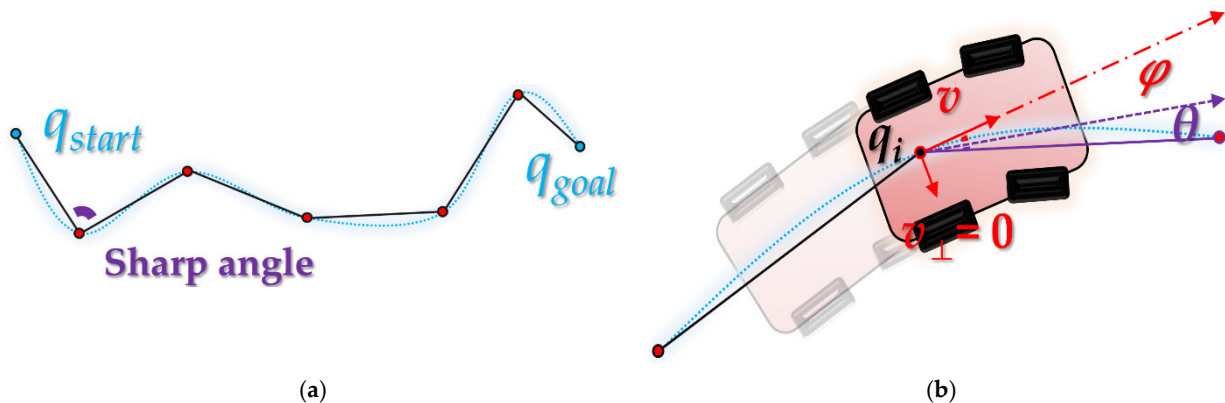
Figure 1. Path of RRT-like algorithms with sharp angle: (a) piecewise linear path; (b) situation with turning radius \phi as per the kinematic constraints of mobile robot with velocity v at node (turn penalty \theta ).
