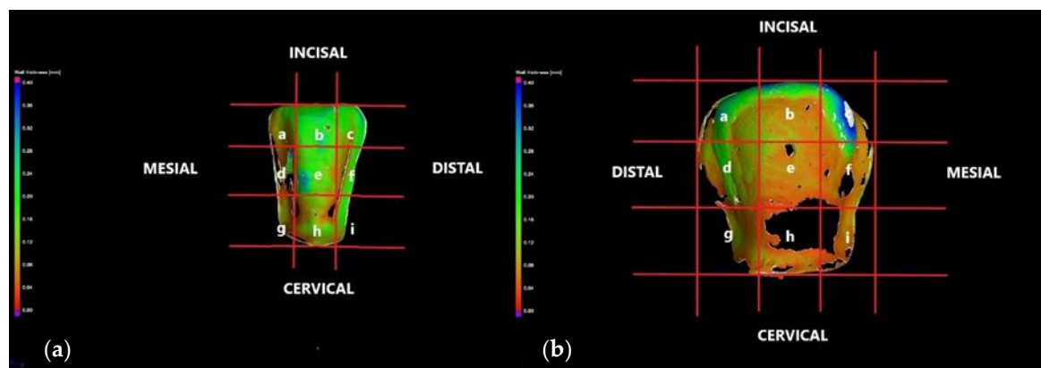
Figure 7. The vestibular face of (a) the CO tooth preparation, displaying the thickness/width w of the luting cement on an upper right lateral incisor and of the (b) CR tooth preparation on an upper left canine, both divided into nine quadrants of measurement: a, b, c, d, e, f, g, h, i.
