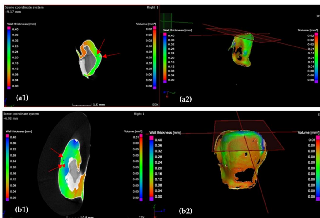
Figure 10. Investigation of the incisal marginal contour of the CO (a) and CR tooth preparation (b) in the transversal plane, displaying a maximum cement width w of 240 \mu\text{m} for the CO and 350 \mu\text{m} for the CR sample. Moreover, porosities (red arrows) are identified at the incisal margins of both preparations. Notations: (1) section and (2) 3D reconstruction.
