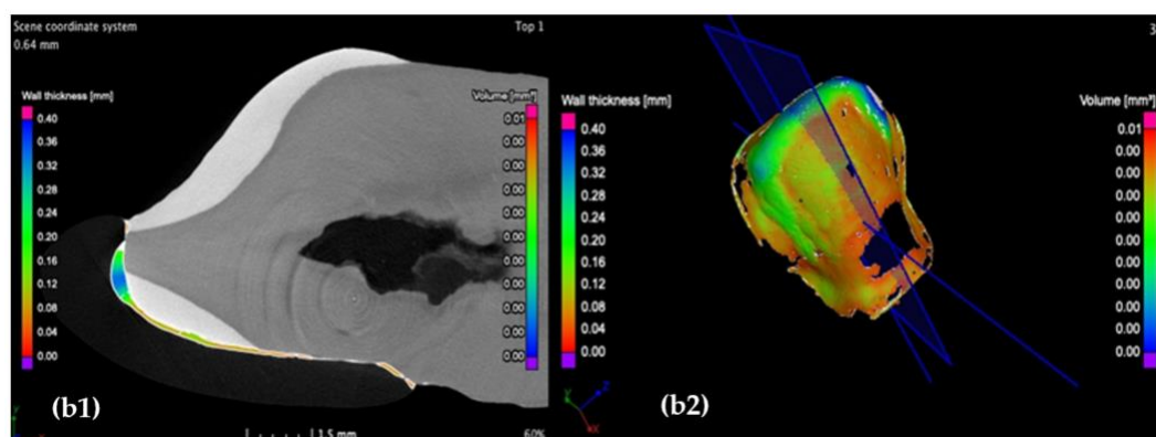
Figure 12. The highest cement thickness/width w situated in the middle of the vestibular face in sagittal section is 280\ \mu\text{m} for (a) the CO and 100\ \mu\text{m} for the CR (b) tooth preparation. Moreover, the layer of the luting cement of the CO sample features porosities within (red arrow) and is less uniform compared to the CR sample. Notations: (1) section and (2) 3D reconstruction.
