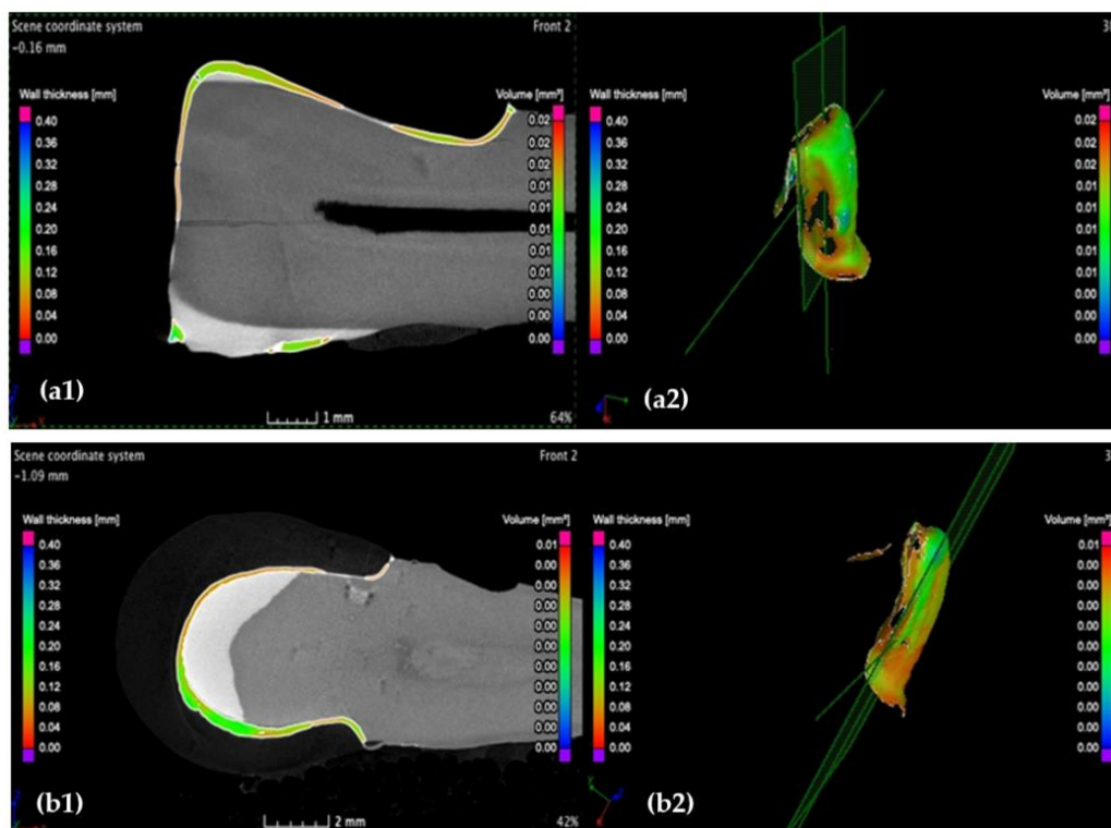
Figure 11. Investigation of the incisal marginal contour of (a) the CO and (b) CR tooth preparation in the frontal plane, displaying a maximum cement width w of 80 \mu\text{m} for both CO and CR samples. Notations: (1) section and (2) 3D reconstruction.
