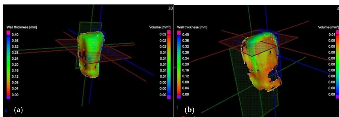
Figure 8. 3D analysis of the wall thickness/width w of samples: (a) CO and (b) CR tooth preparation, displaying the dimension scale (in a color code) on the left side.
