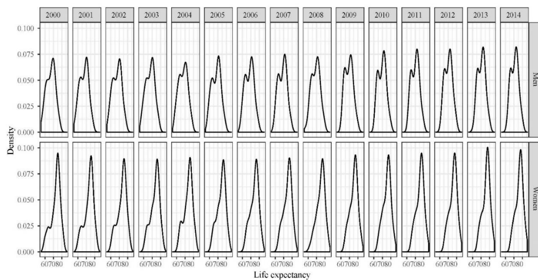
Figure S1. Probability density of life expectancy in B&R countries.
