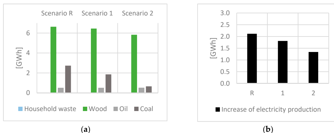
Figure 14. (a) Results showing the fuel use of the DHC system productions units in order to satisfy the demand of the HPS for each scenario. Results are presented relative to a scenario where no HPS are used and conventional snow clearance must be used. (b) Results showing the increase in electricity production at the CHP plants for each scenario.
