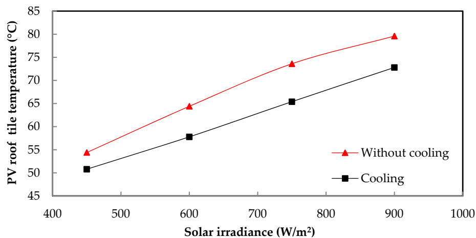
Figure 6. The PV roof tile temperature variation with the solar irradiance, with the cooling air flow rate at \dot{V} = 5 m 3 /h.
