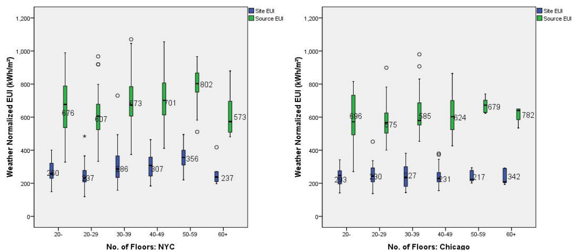
Figure 7. Site and source energy use intensity per number of floors.
