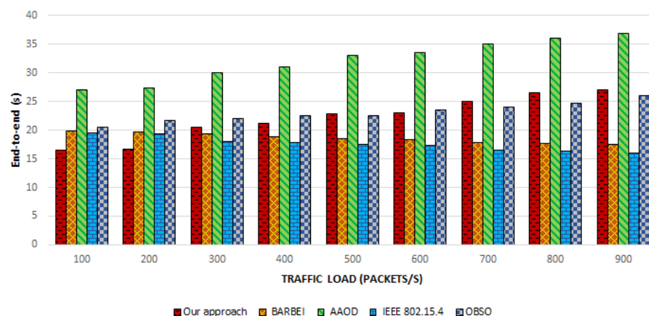
Figure 7. End-to-end delay.
