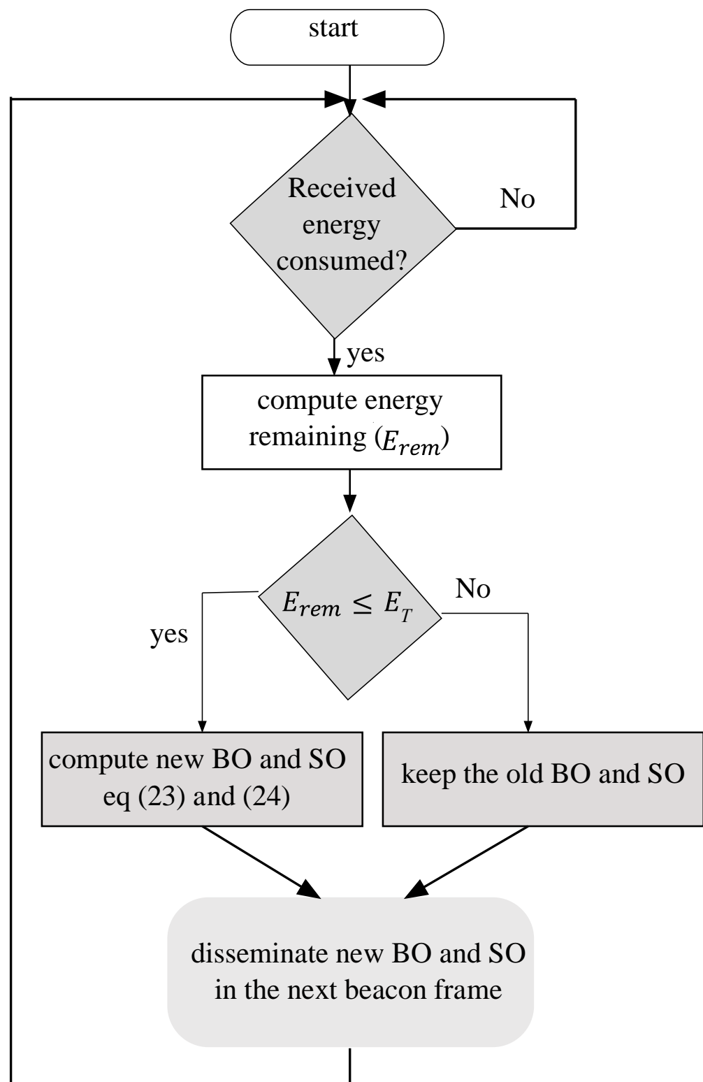
Figure 4. Flowchart of duty-cycle adjustment algorithm for IEEE 802.15.4.
