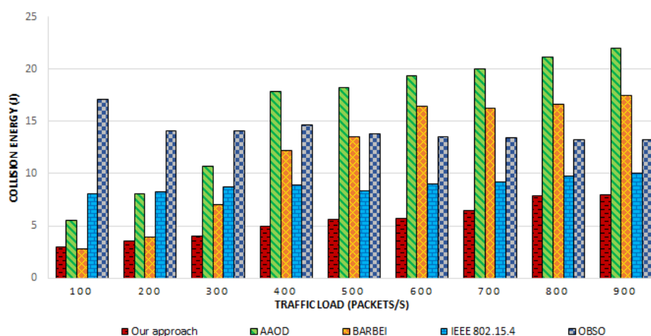
Figure 8. Collision energy consumption.
