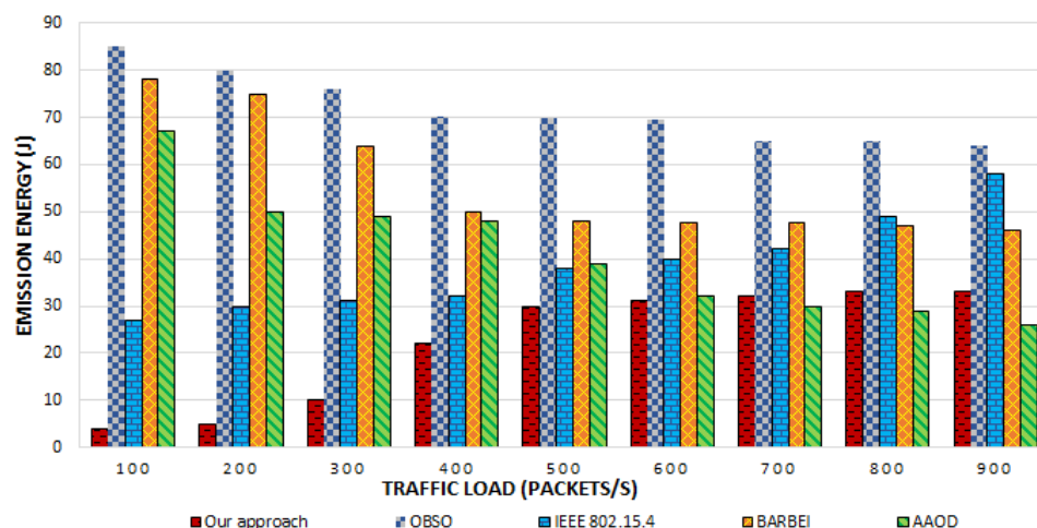
Figure 9. Emission energy consumption.
