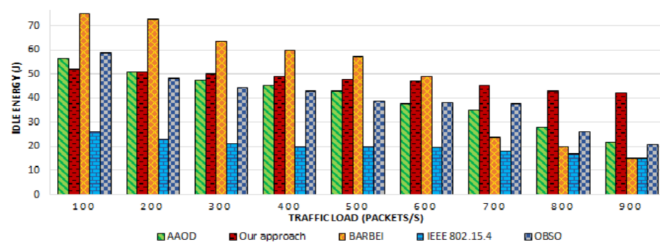
Figure 13. Idle energy consumption.
