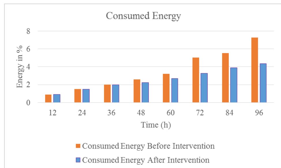
Figure 17. Energy consumption.
