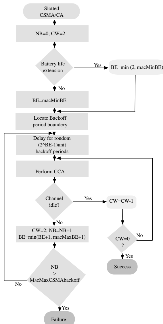
Figure 3. Flowchart of slotted CSMA/CA algorithm for IEEE 802.15.4.
