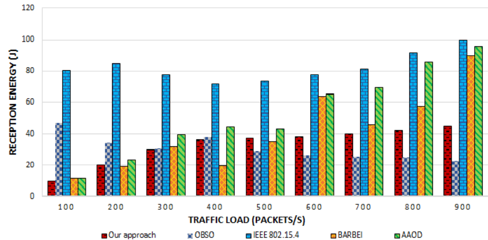
Figure 11. Reception energy consumption.
