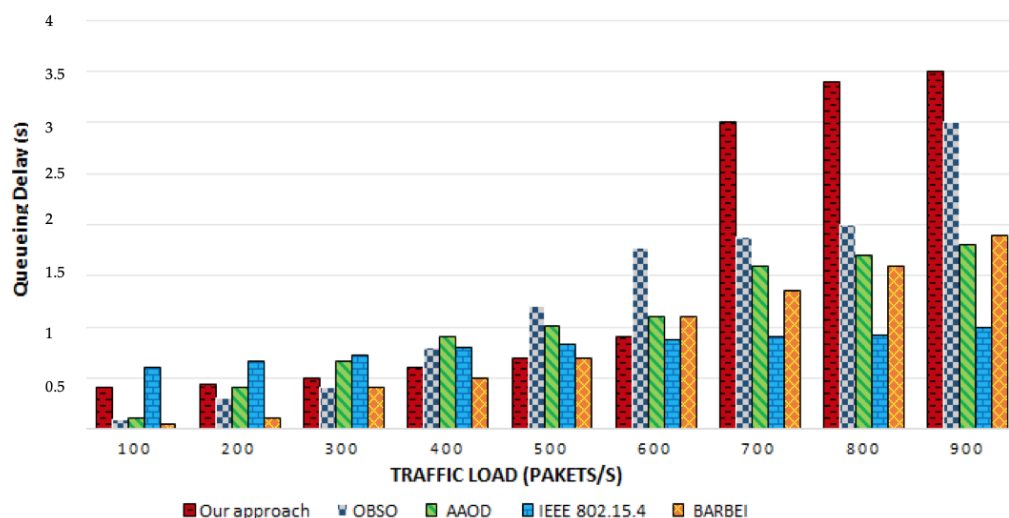
Figure 6. Queueing delay.
