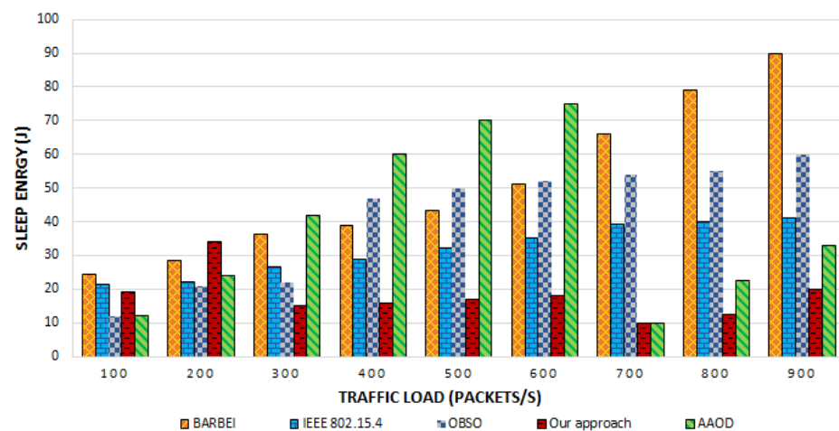
Figure 12. Sleep energy consumption.
