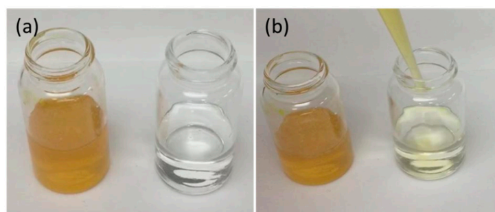
Figure S2. The color change in the acetylsalicylic acid solution released by gel-3 before (a) and after (b) the addition of FeCl 3 .
