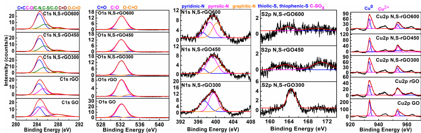
Figure S2. XPS spectra for graphene coatings.
