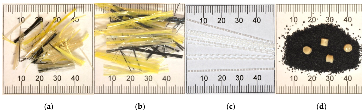
Figure 3. The additives used in the tests: (a) 19-mm-long aramid fibres; (b) 38-mm-long aramid fibres; (c) 50-mm-long polymer fibres, and (d) crumb rubber and polyoctyner polymer modification applied to bitumen.
