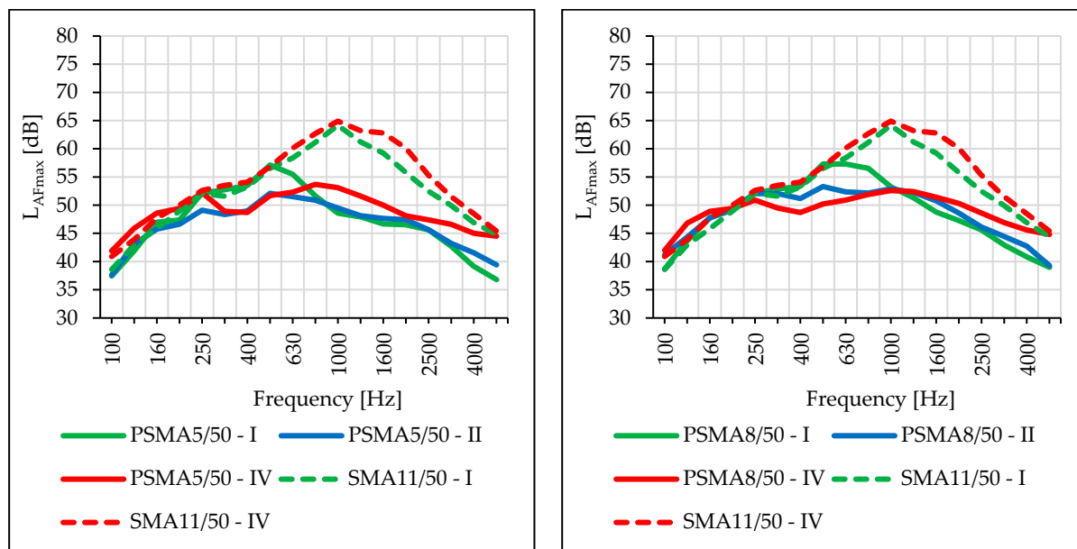
Figure 28. Comparison of sound spectra from a statistical passenger vehicle depending on the period of road use (PSMA5 and PSMA8).
