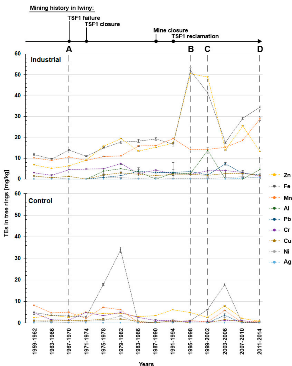
Figure 3. Historical variations of selected trace elements (TEs) in the tree rings of pedunculate oak in different study sites (Control vs. Industrial (Ind.)) between 1959 and 2014. Vertical dashed lines indicate the time intervals (A-D) that have been selected for verification by inductively coupled plasma mass spectrometry (ICP-MS).
