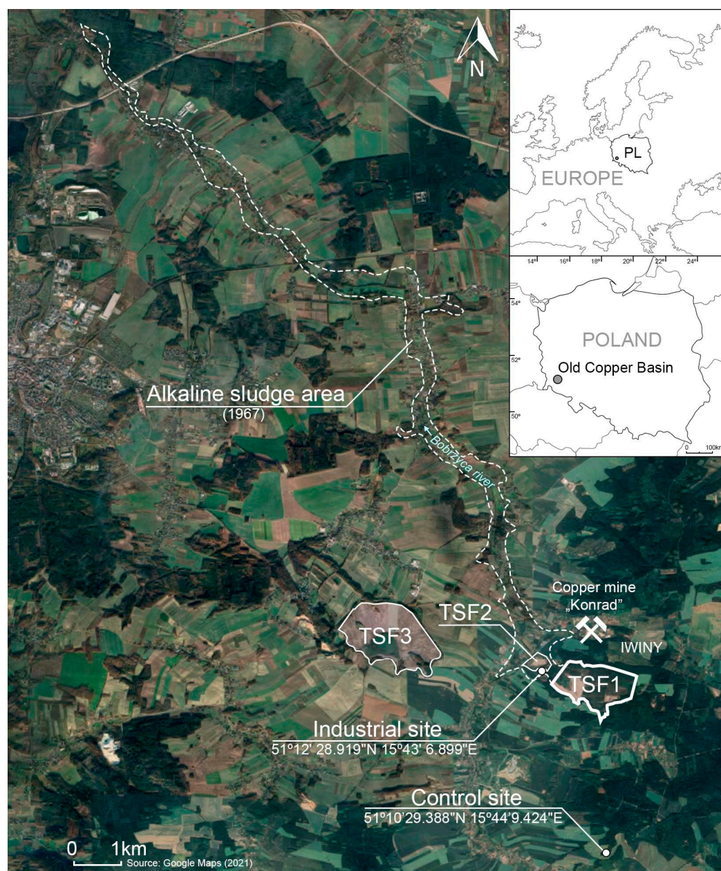
Figure 1. Location of study plot: Industrial (Ind.) and Control site and tailings storage facilities (TSFs) in so-called Old Copper District, Poland. The 1967 leakage area is presented on the basis of materials from the State Archive in Wrocław, Bolesławiec Branch [53].
