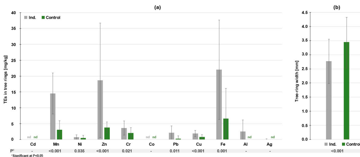
Figure 2. (a) Mean trace element (TE) contents [mg/kg] in the tree rings of pedunculate oak in different study sites (Control vs. Industrial (Ind.)) between 1959 and 2014 (with standard deviation ( \pm SD) error bars). Values below the limit of detection (LOD) were marked as nd (not detected); (b) Mean tree rings' widths (TRWs) of trees growing at the Iwiny Industrial and Control site between 1959 and 2014 (with standard deviation ( \pm SD) error bars).
