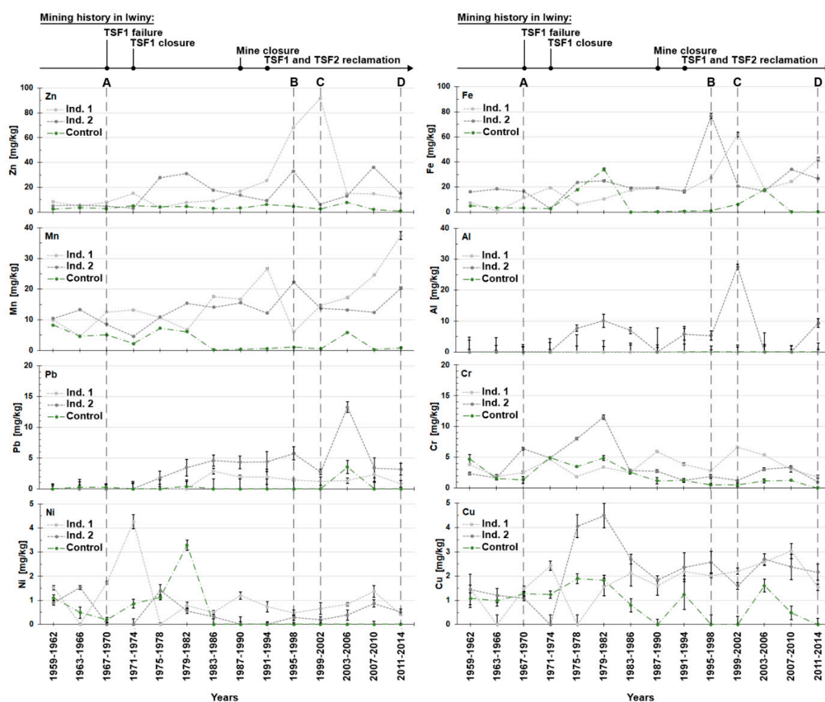
Figure 4. Trace elements (TEs) contents [mg/kg] in tree rings of all studied trees: Industrial 1 (Ind. 1), Industrial 2 (Ind. 2), and Control from 1959 to 2014. Vertical dashed lines indicate the time intervals (A–D) verified by inductively coupled plasma-mass spectrometry (ICP-MS).
