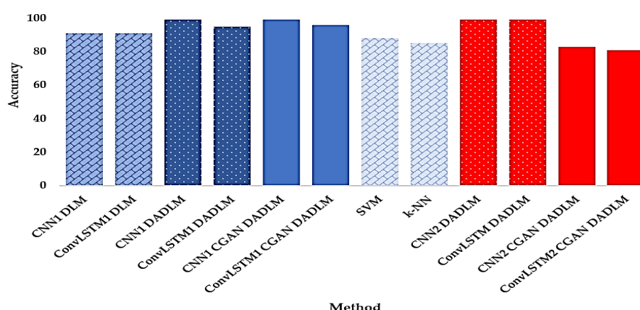
Figure 33. Performance comparison of the proposed DLMs for different datasets.
