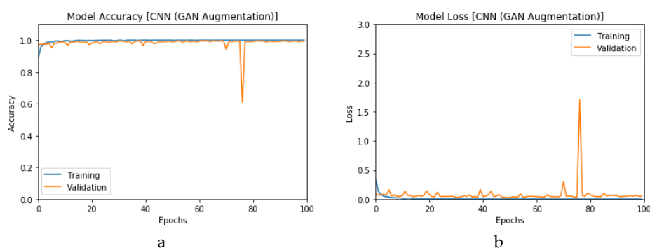
Figure 24. Outcomes for CNN 1 CGAN DADLM with prior GAN data augmentation for the first dataset showing (a) Accuracy and (b) Logarithmic loss.
