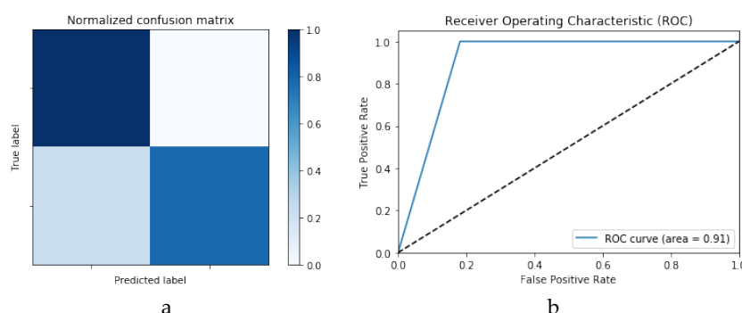
Figure 15. Outcomes for ConvLSTM 1 DLM without data augmentation for the first dataset showing (a) Confusion matrix and (b) ROC curve
