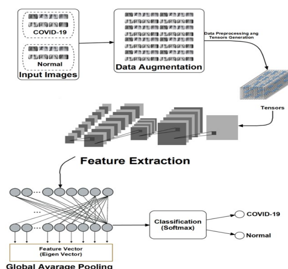
Figure 1. Architecture showing data flow in the proposed image transformation deep learning models (DLMs).
