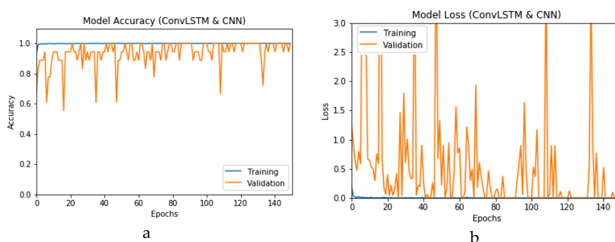
Figure 17. Outcomes for ConvLSTM 1 DADLM with prior data augmentation for the first dataset showing (a) Accuracy and (b) Logarithmic loss.
