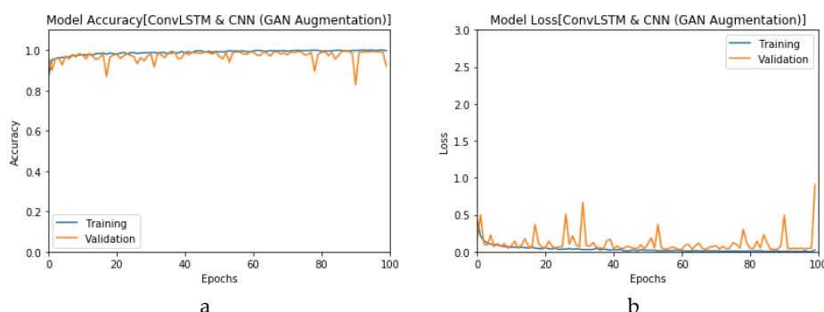
Figure 25. Outcomes for ConvLSTM 1 CGAN DADLM with prior GAN data augmentation for the first dataset showing (a) Accuracy and (b) Logarithmic loss.
