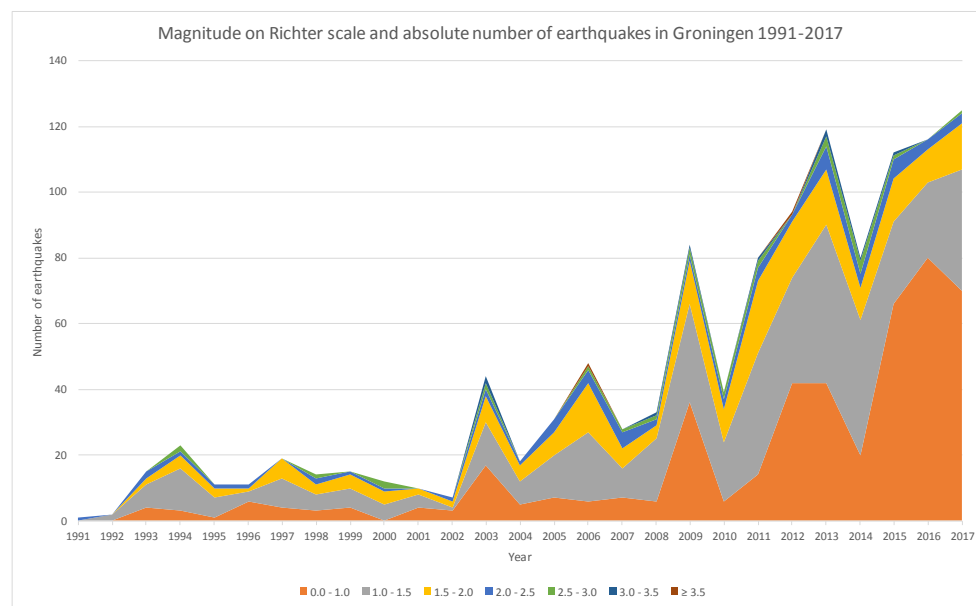
Figure 2. The magnitude and number of earthquakes in Groningen (source: authors, based on data from NAM [66]).
