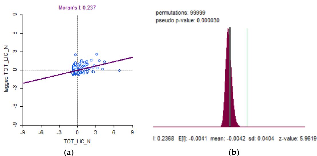
Figure 2. Moran’s I Test Statistics for the number of radioactive materials licenses. (a) Moran’s I scatter plot for the number of radioactive materials (Moran’s I = 0.237); (b) Reference distribution for Moran’s I (pseudo p -value = 0.000030). (Note: TOT_LIC_N = number of radioactive material licenses in a region; lagged TOT_LIC_N = the average number of radioactive material licenses in the neighboring regions of a region.).
