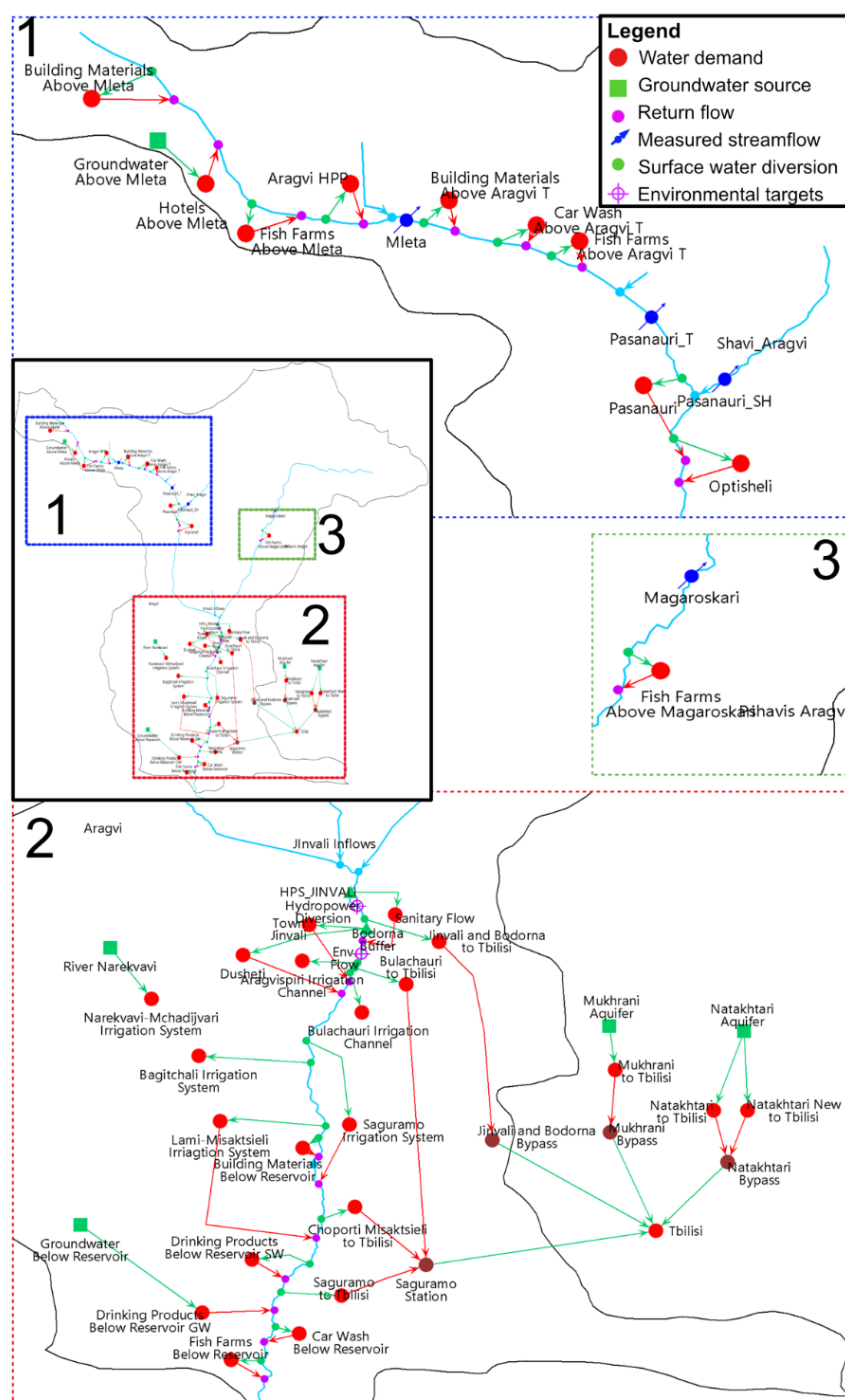
Figure 2. Model Schematic from WEAP. This schematic show only approximate location of water demands, groundwater sources, return flows, streamflow gages, and surface water diversion in the system. Note: the location of Tbilisi do not correspond with actual location which is further downstream.
