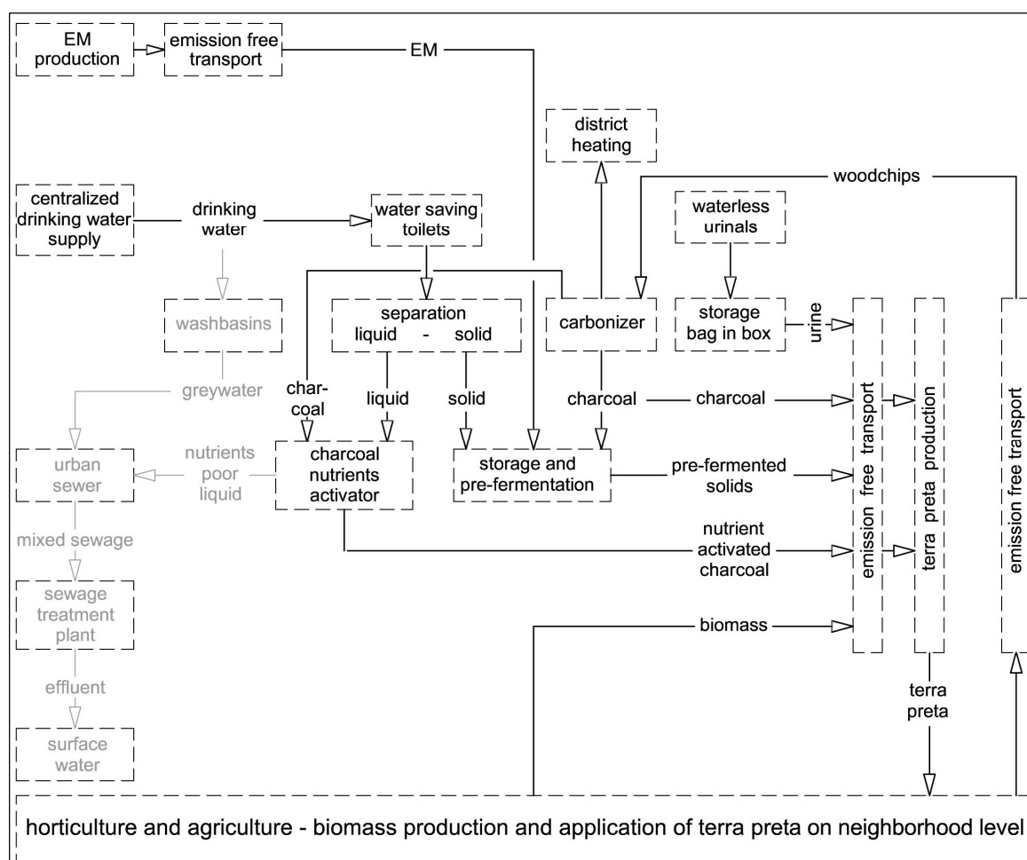
Figure 3. Flowchart of TPS System of the TerraBoGa project, illustrating the connections between processes and/ or technologies (in boxes) and resulting products (without boxes). All processes except the steps after the discharge of grey water and liquids in the sewer system occur within the botanic garden.
