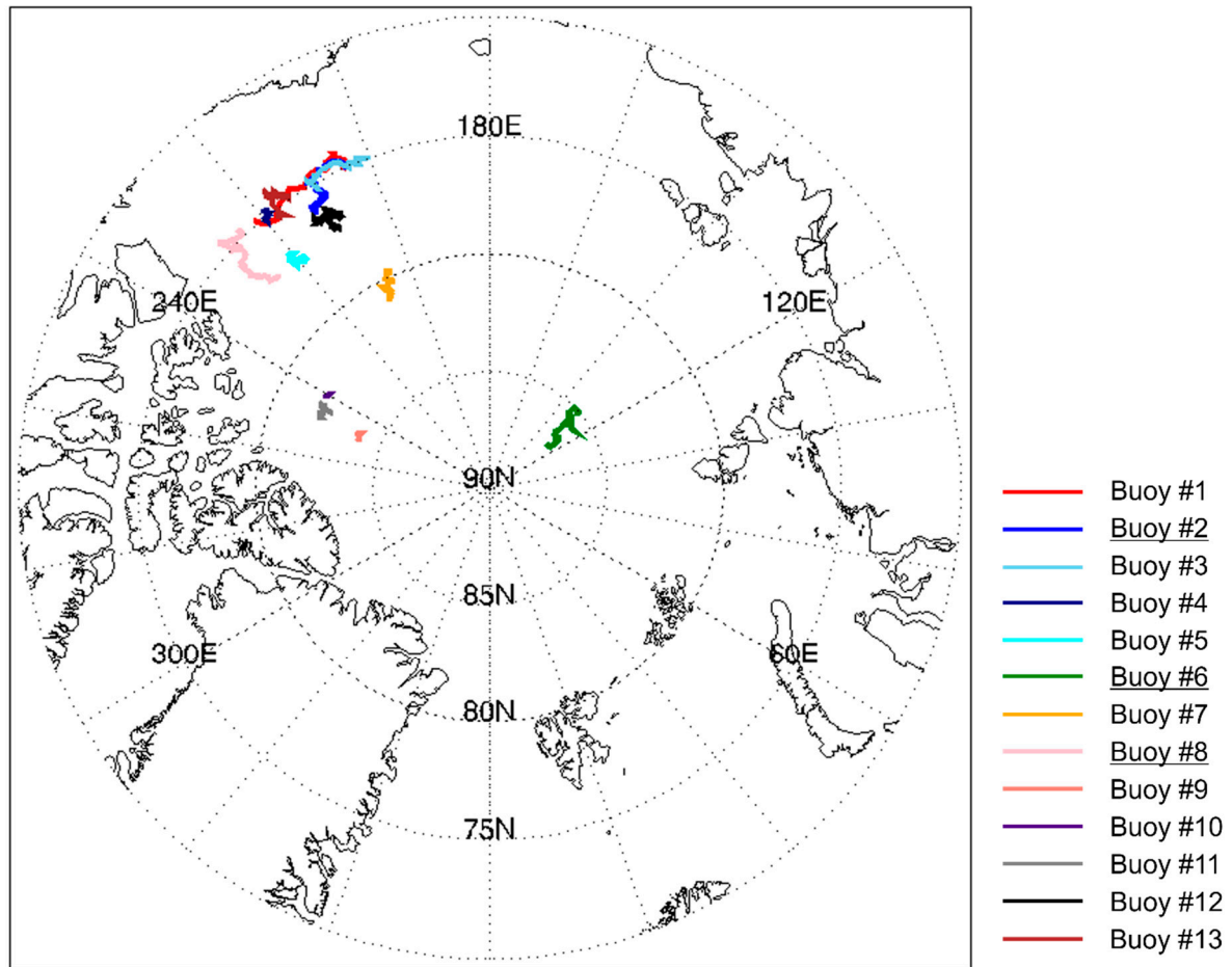
Figure S1. Tracks of the 13 selected buoys deployed in the Arctic sea. Colors indicate different buoy tracks, and numbers correspond to deployed buoys defined in Table 3. Three rejected buoys (#2, #6, and #8) are underlined in the labels.
