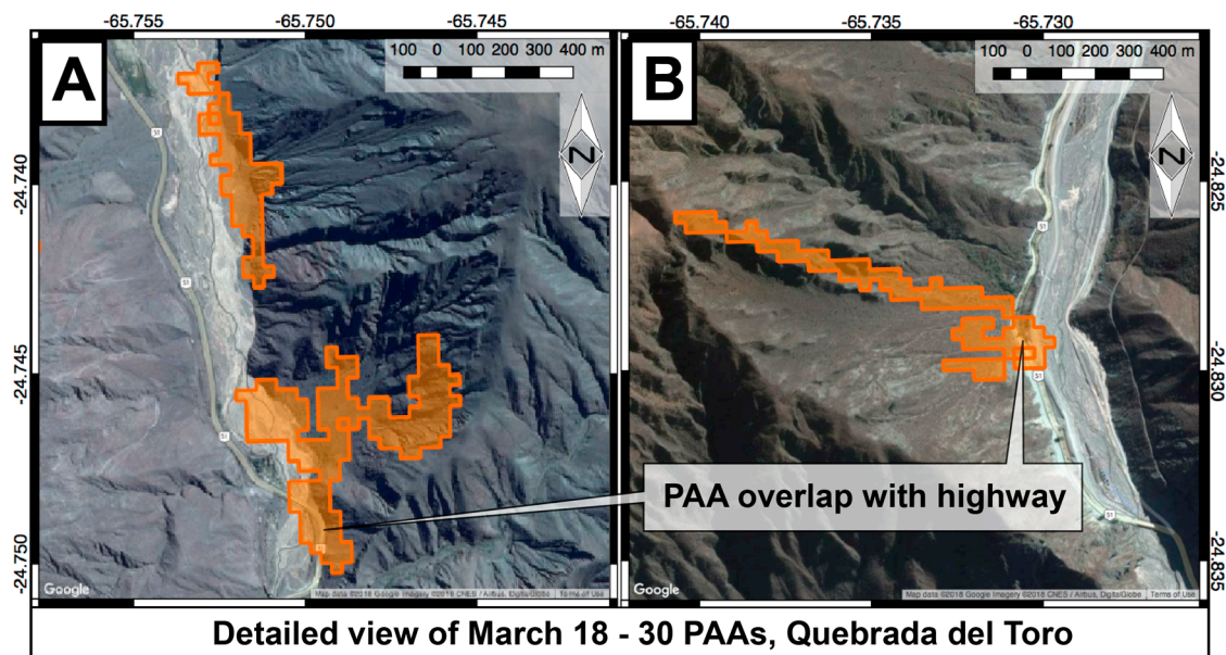
Figure 7. Details of PAA overlap with highway infrastructure. Satellite optical images from this time are obscured by cloud cover, but detected PAAs are located downslope of scree slopes and gullying (A) and high-relief surfaces (B) with potential for landslides or mudflows. Satellite imagery from Google Earth Pro, CNES/Airbus, and Digital Globe.
