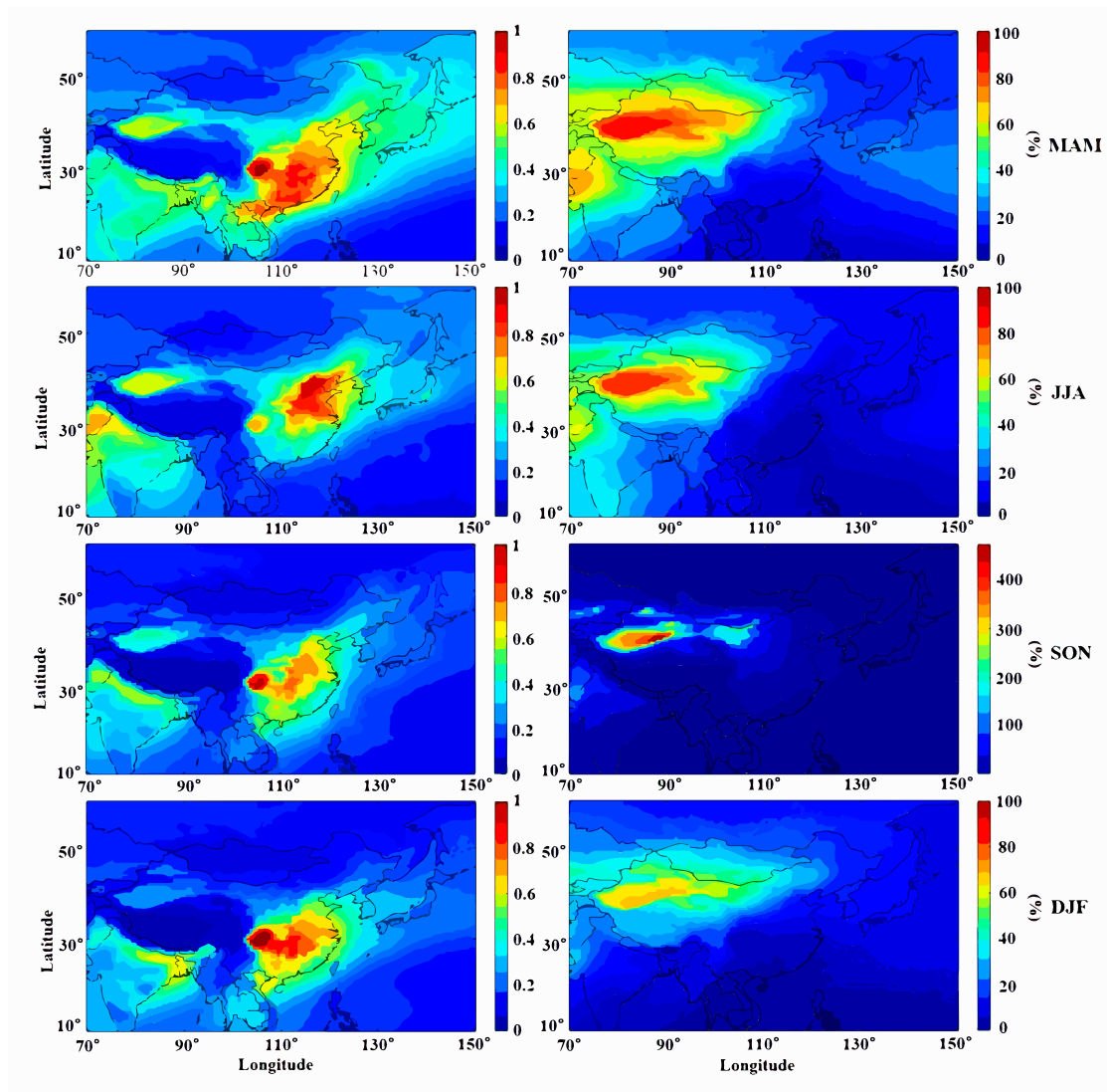
Figure S1: Seasonal distribution of Aerosol Optical Depth (left panels) and percentage contributions of pure dust to the total AOD (right panels) over East Asia based on MERRA-2 data
