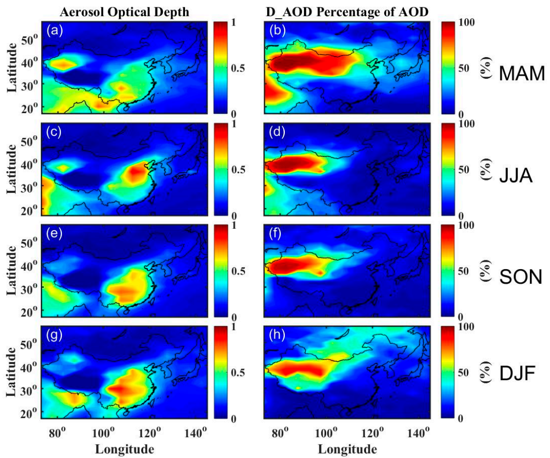
Figure S2: Seasonal distribution of Aerosol Optical Depth (left panels) and percentage contributions of pure dust to the total AOD (right panels) over East Asia based on CALIPSO data
