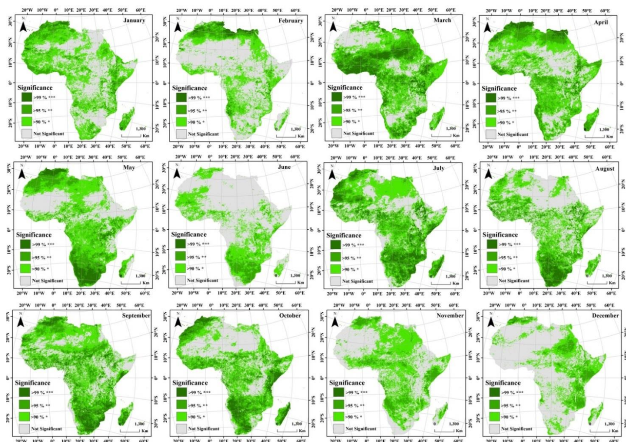
Figure S4. Significance of the spatial distribution of monthly LST trends in Africa from 2003 to 2017.
