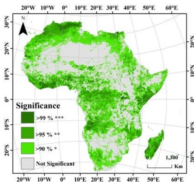
Figure S1. Significance of the spatial distribution of annual LST trends in Africa from 2003 to 2017. The symbols ***, **, and * represent significant warming/cooling trends at the 99%, 95% and 90% confidence levels based on an independent-samples t-test, respectively (same as below).
