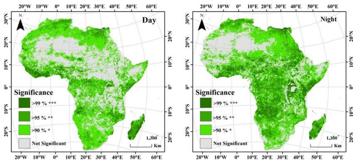
Figure S2. Spatial dynamics of the significant diurnal variations in diurnal LST change from 2003 to 2017.
