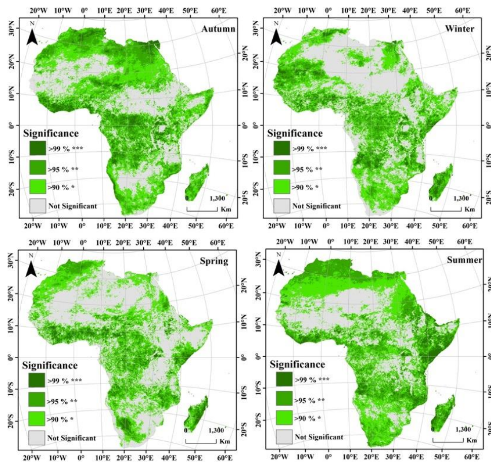
Figure S3. Significance of the spatial distribution of seasonal LST trends from 2003 to 2017.
