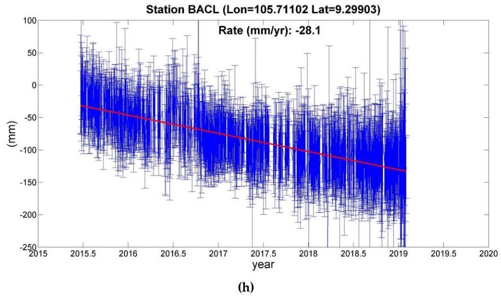
Figure S1. Time-series of heights plots of 8 stations provided by the Institute of Geophysics (IGP) – Vietnam Academy of Science and Technology (VAST) (a) MTEV station; (b) MLAY station; (c) DBIV station; (d) SMAV station; (e) PHUT station; (f) VINH station; (g) HUES station and (h) BACL station.
