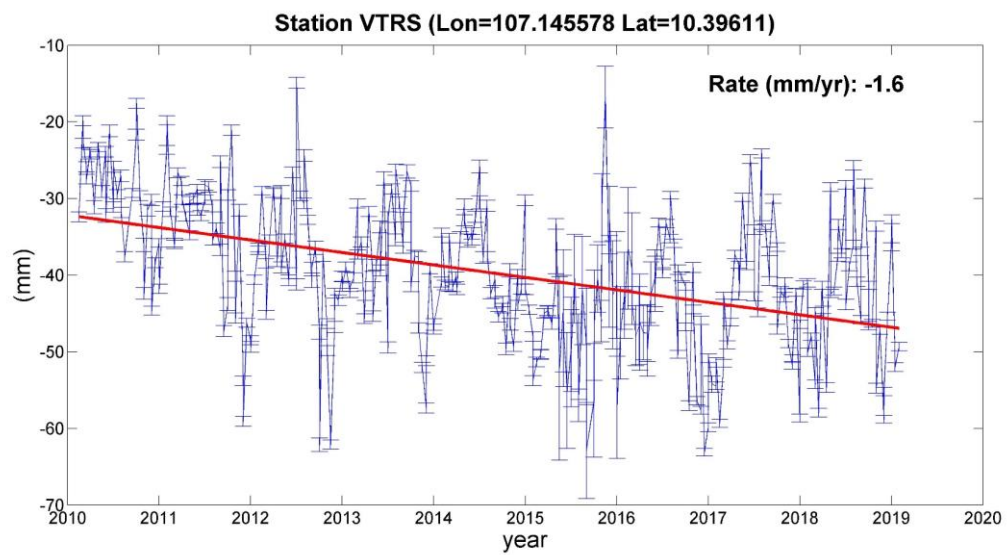
Figure S2. Time-series of heights plots of 3 stations provided by the Vietnam Department of Surveying and Mapping (VDSM) (a) DSRS station; (b) QNRS station and (c) VTRS station.
