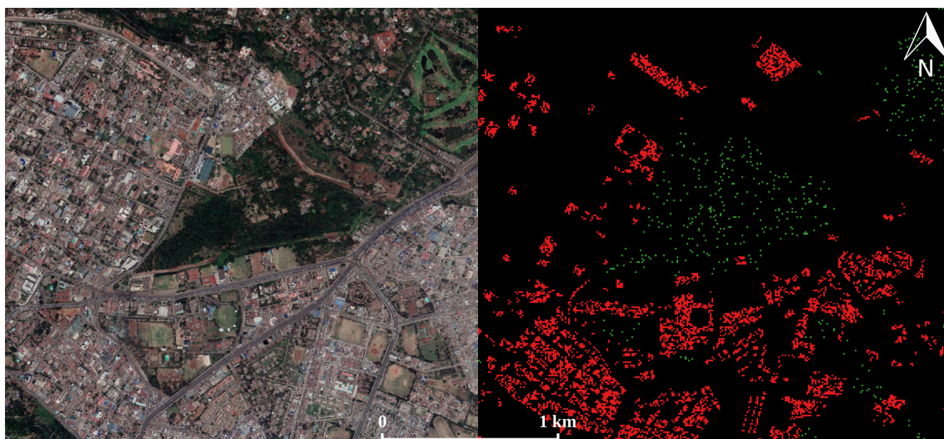
Figure 4. Training samples collected from OSM in Nairobi, Kenya. (a) Aerial view of the area of interest, courtesy of Google Earth; (b) built-up (red) and non-built-up (green) training samples over the same area of interest.
