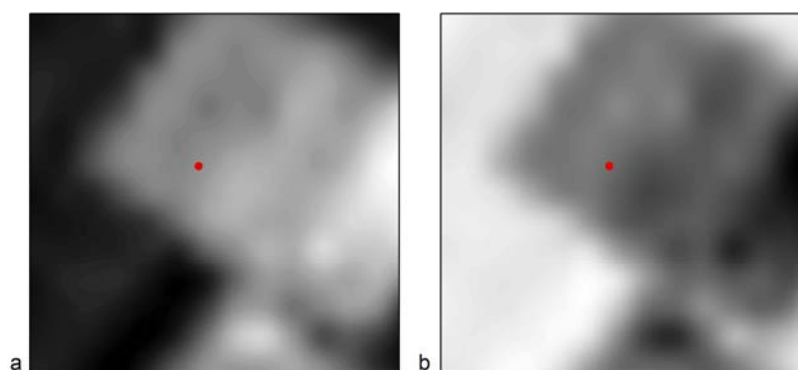
Figure 9. Landsat multispectral images used for the detection of the neolithic tell Melia 2 (indicated with a red spot) at the Thessalian plain, after the application of broadband indices: (a) EVI and (b) Green NDVI.
