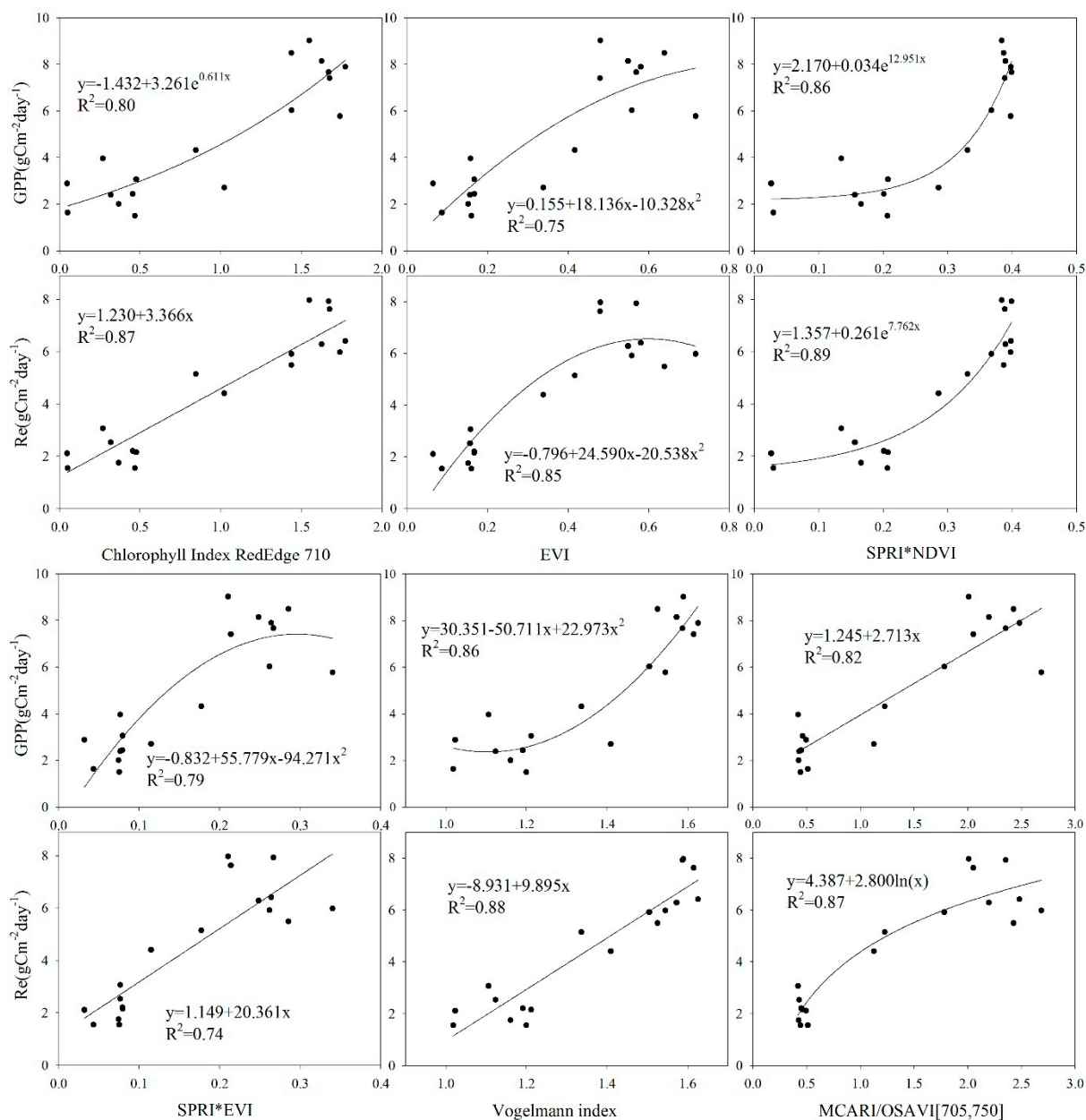
Figure 8. Scatter plots of 6 bio-indicators and measured GPP and Re. All fitting models are significant at the 0.01 level (2-tailed).
