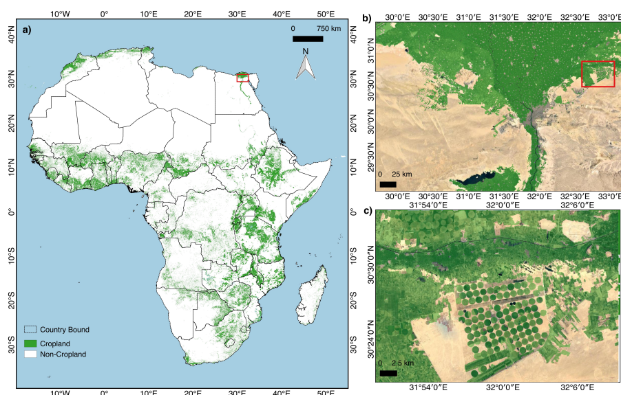
Figure 6. Global Food Security-support Analysis Data @ 30-m of Africa, Cropland Extent product (a). Full resolution of 30-m cropland extent can be visualized by zooming-in to specific areas as illustrated in right panel (b,c). For any area in Africa, croplands can be visualized by zooming into specific areas in croplands.org .
