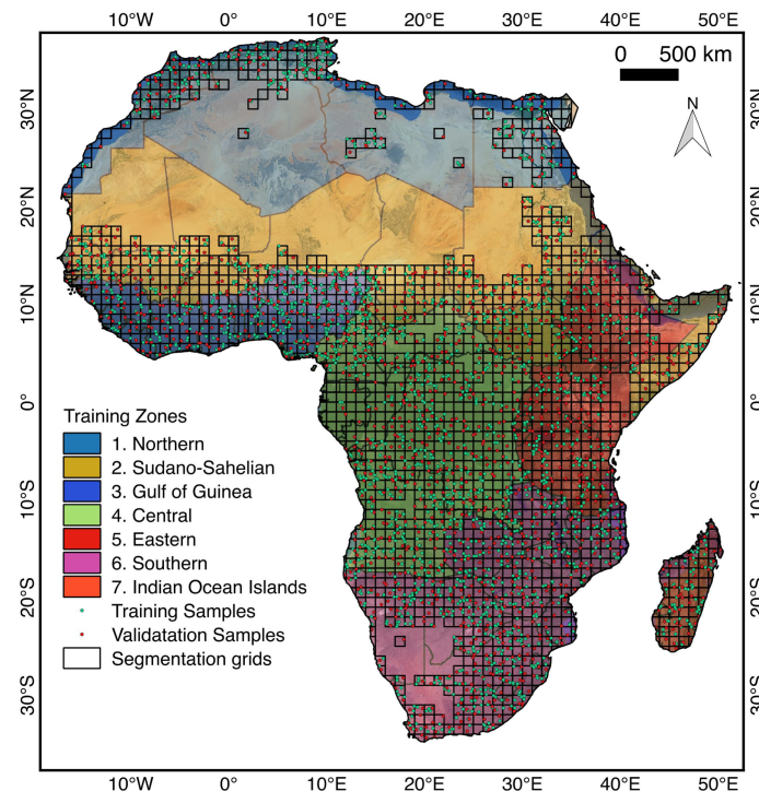
Figure 1. Map of Africa and its seven stratified zones used in the study. The pixel-based supervised classifications were run separately for each of the 7 refined agro-ecological zones (RAEZs, or simply referred to as zones: Northern, Sudano-Sahelian, Gulf of Guinea, Central, Eastern, Southern, Indian Ocean Islands). The object-based segmentation was run on each 1^\circ \times 1^\circ grids to delineate crop field boundaries. The dots represent the location of the reference training and validation samples (green indicates training and red indicates validation).
