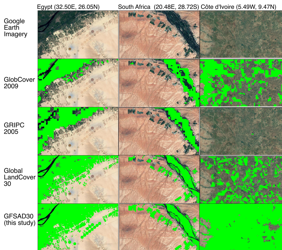
Figure 8. A visual comparison of all crop extent products (shown in green) overlaid on Google Earth Imagery.
