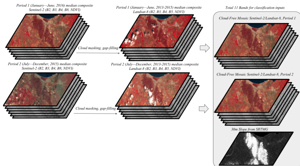
Figure 2. Illustration of the 11 input layers in this study. Five bands (Blue, Green, Red, NIR, NDVI) were composited for each of two periods (period 1: January–June 2016, and period 2: July–December 2015) for entire African continent. Total 10 bands plus the slope layer derived from SRTM elevation data were composed on GEE for pixel-based classification, 10 bands without slope layer were used for object-based segmentation.
