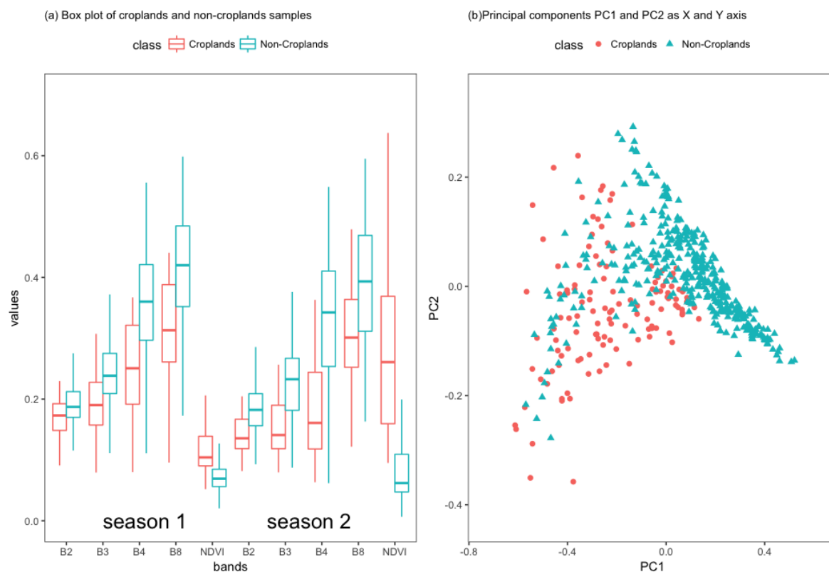
Figure 3. Creating knowledge-base to separate croplands from non-croplands involving: (a) waveband reflectivity and NDVI of the two seasons; and (b) principal component plot. The above knowledge-base is illustrated for a sub-area in one of the seven zones shown (Figure 1) of Africa.
