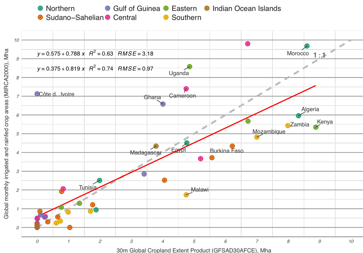
Figure 7. Scatter plot of GFSAD30AFCE derived cropland areas versus MIRCA2000 (Personal communication with Dr. Siebert and Dr. Portmann by Dr. Thenkabail) derived cropland areas country by country for Africa.
