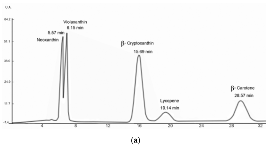
Figure S3. Chromatograms obtained for carotenoid analysis by HPLC-UV-visible: (a) Commercial standards; (b) Extract of destringed persimmon fruit 'Rojo Brillante' PDO 'Ribera del Xúquer'. Chromatographic conditions: see text.
