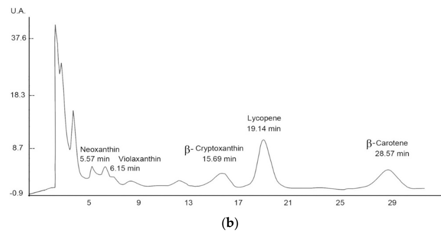
Figure S3. Chromatograms obtained for carotenoid analysis by HPLC-UV-visible: (a) Commercial standards; (b) Extract of destringed persimmon fruit 'Rojo Brillante' PDO 'Ribera del Xúquer'. Chromatographic conditions: see text.
