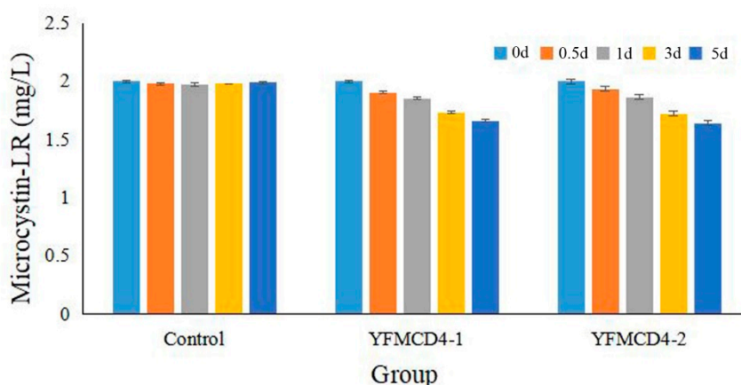
Figure S1. The degradation activities of MC-LR by YFMCD4-1 and YFMCD4-2.
