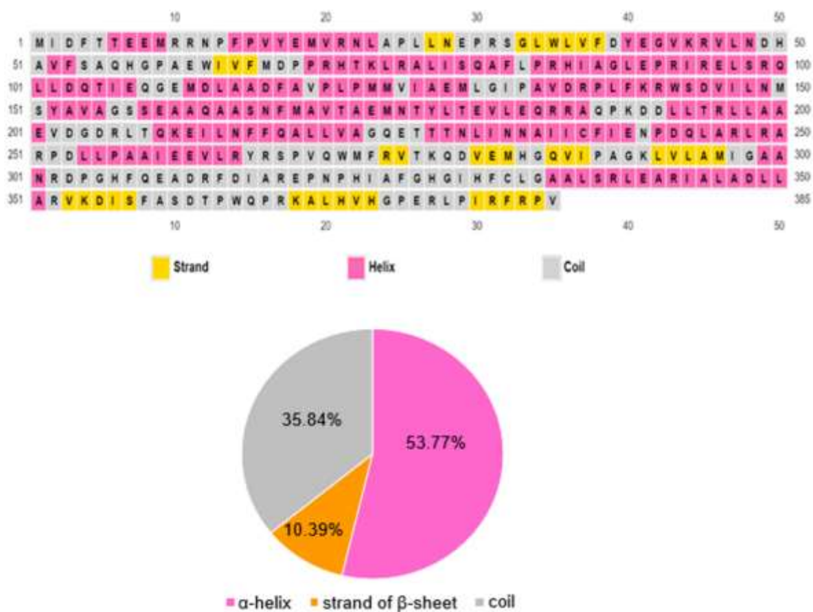
Figure S2. Prediction of secondary structures of P450-T3 using the PRIPRED tool.
