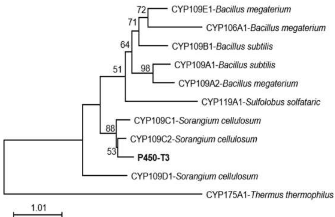
Figure S1. Phylogenetic tree of P450-T3 in the cluster of the CYP109 family. Evolutionary analyses were conducted in MEGA X.
