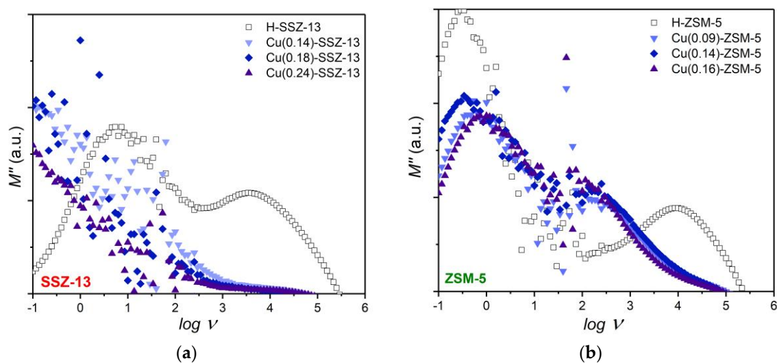
Figure S1. Modulus plots of in situ IS results collected in N 2 at 200 °C over H-form and Cu-exchanged (a) SSZ-13 and (b) ZSM-5 zeolites.
