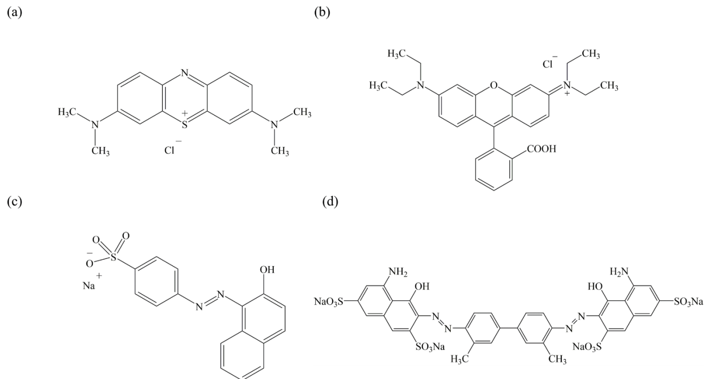
Figure S1. Chemical structures of dyes: (a) methylene blue (MB); (b) Rhodamine B (RhB); (c) Orange II (OI); (d) trypan Blue (TB).
