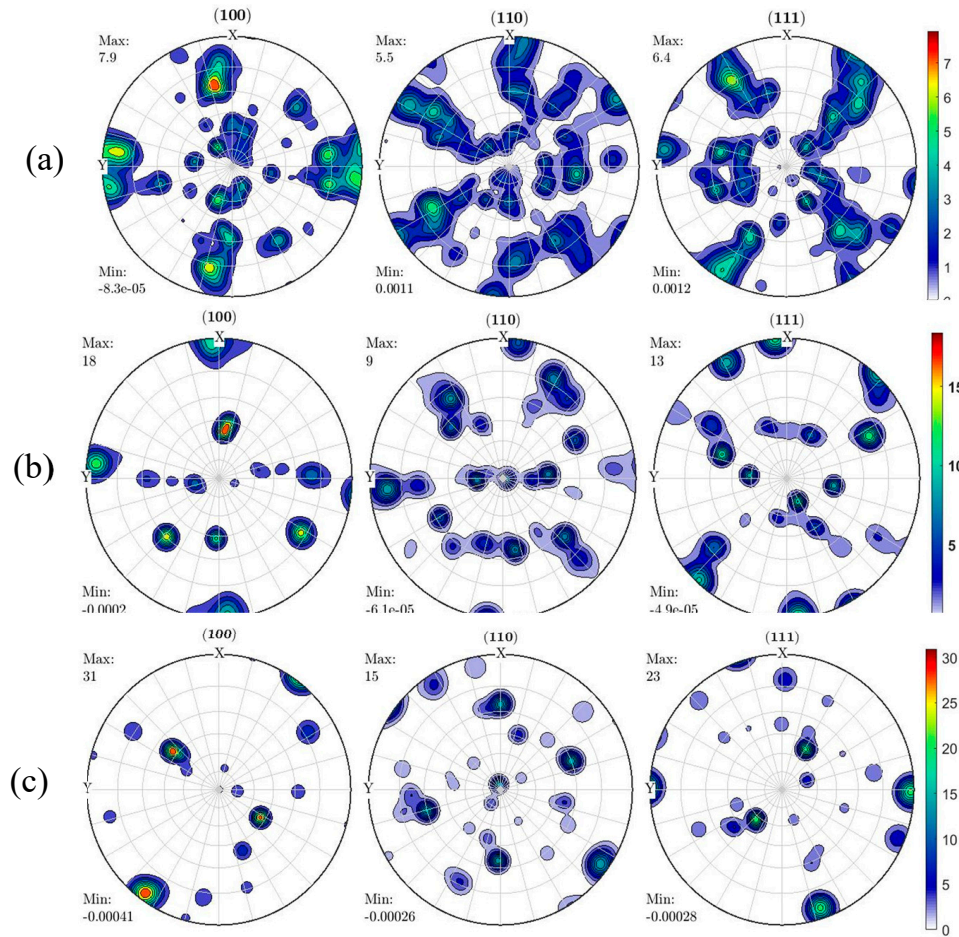
Figure 11. The (100), (110), and (111) pole figures of the reconstructed \beta -phase of (a) samples A, (b) samples B, and (c) samples C.
