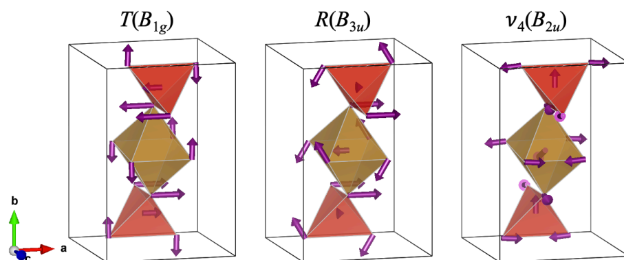
Figure 7. Eigenvectors of the phonon frequencies with negative pressure coefficients of \text{FeVO}_4\text{-II} . We used the VESTA software [46] to build the structures.
