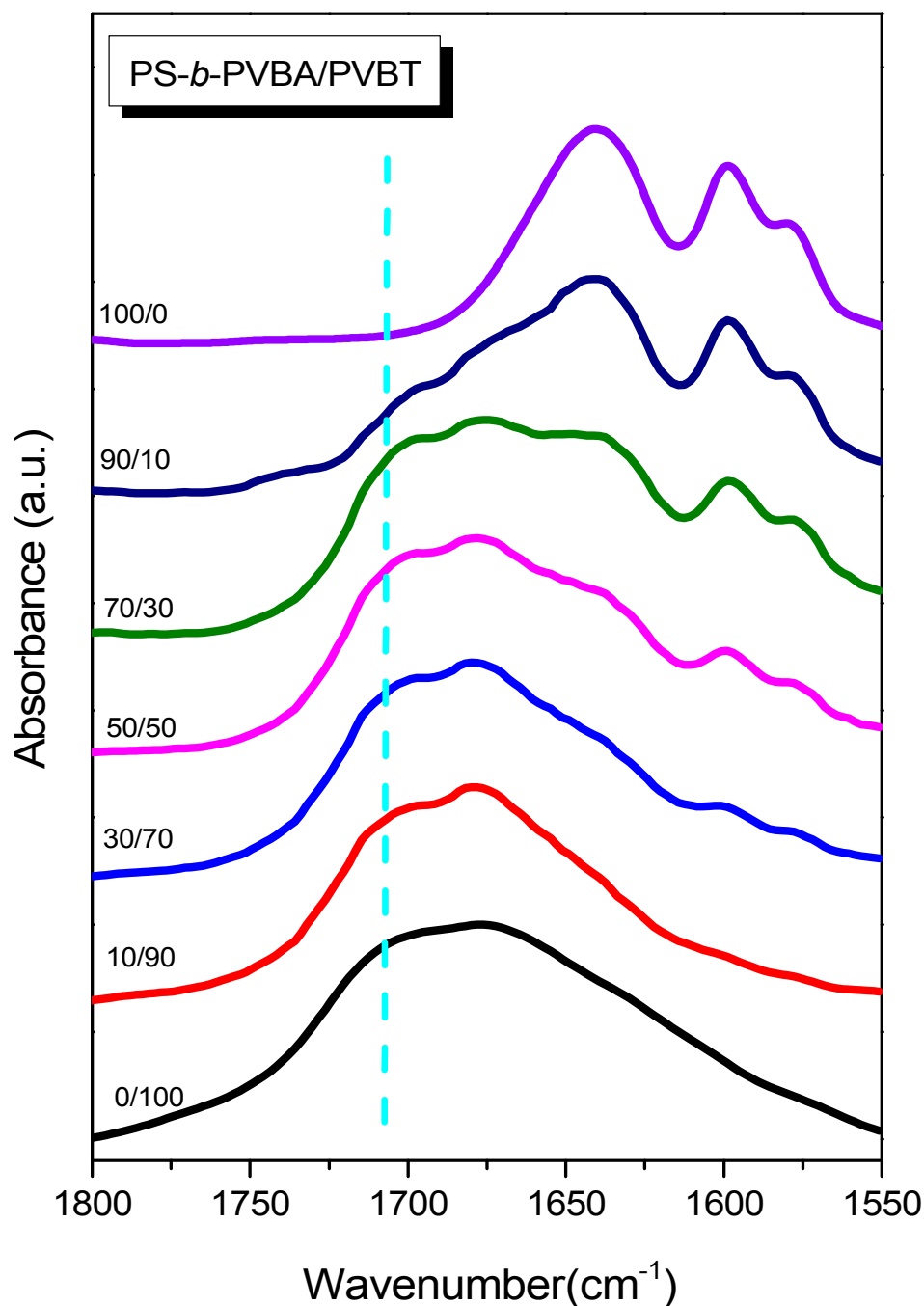
Figure S1. Scale expanded FTIR spectra of PS- b -PVBA/PVBT diblock copolymer/homopolymer blends with various compositions based on Figure 6.
