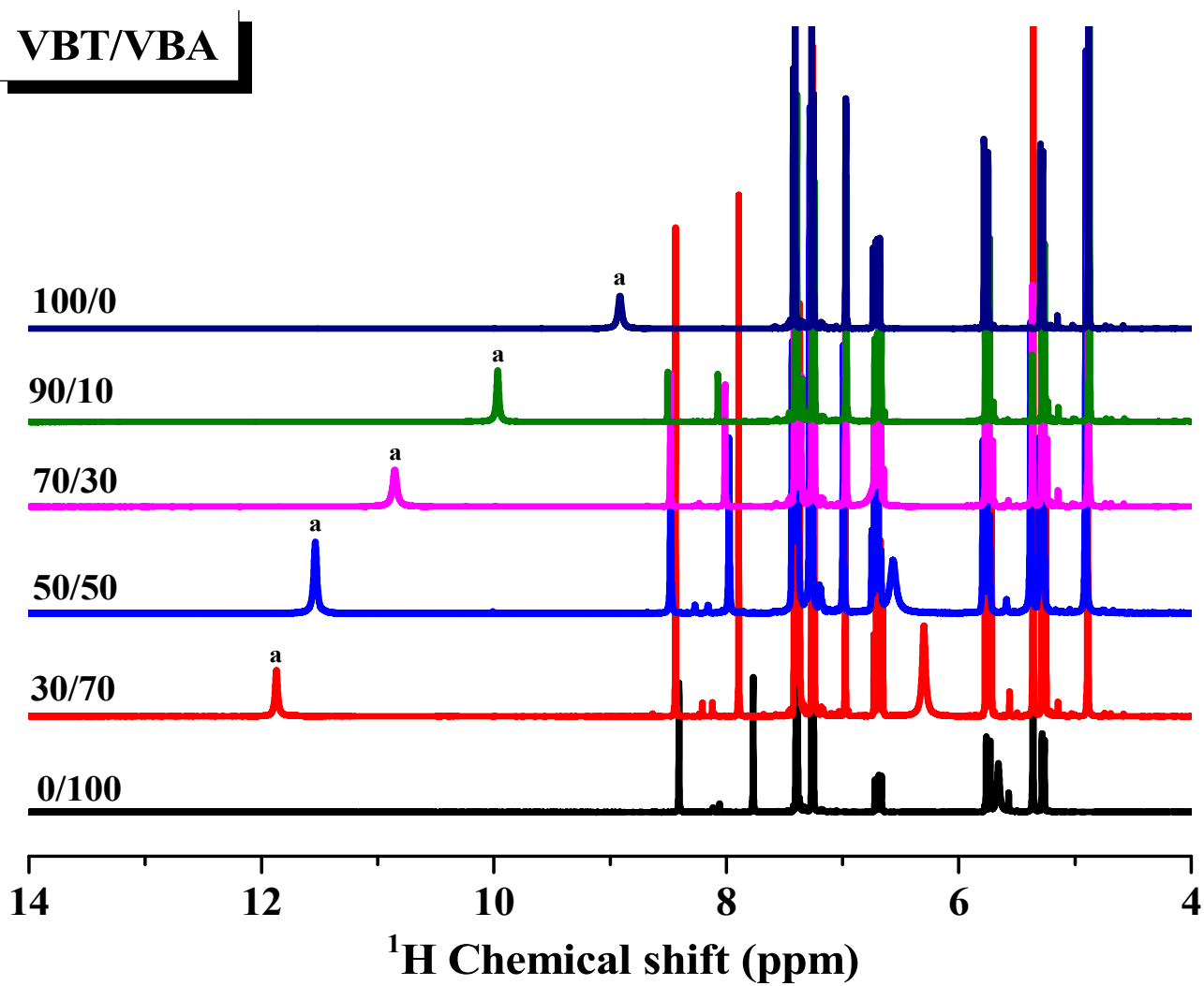
Figure S2. ^1\text{H} NMR spectra displaying the chemical shift of the NH groups of VBT/VBA mixtures of various compositions.
