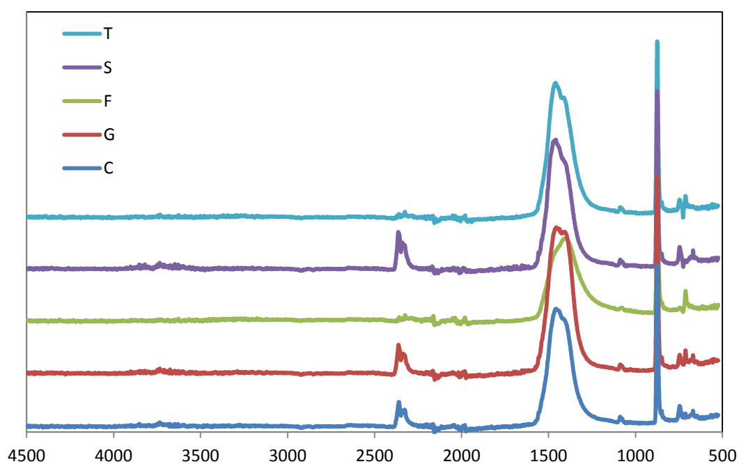
Figure S1. FTIR spectra of calcium carbonate precipitated without additives (C), with glucose (G), fructose (F), sucrose (S), and trehalose (T).
