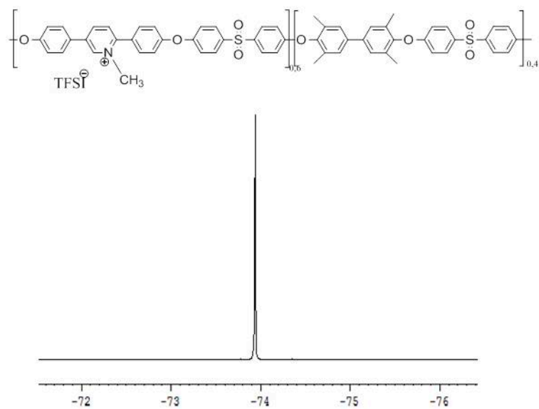
Figure S1. ^{19}\text{F} NMR spectrum for PIL containing TFSI ^{-} as counter anion.
