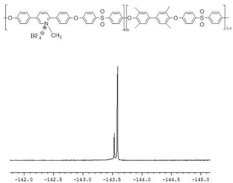
Figure S2. ^{19}\text{F} NMR spectrum for PIL containing \text{BF}_4^- as counter anion.
