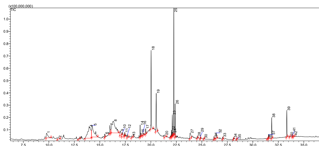
Figure 5. GC/MS chromatogram (in TIC mode) of C. hissaricus extract.
