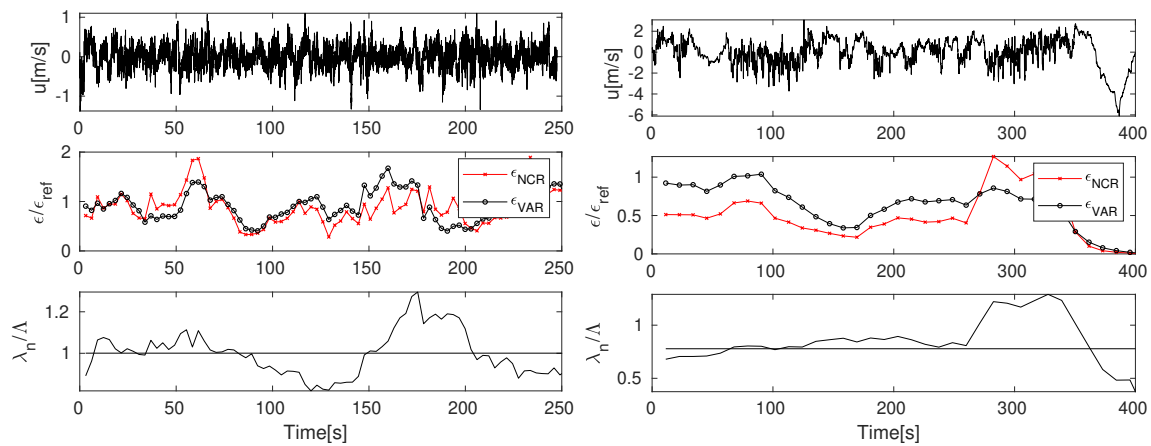
Figure 28. Top plots: Part of the POST signals, middle plots: \epsilon estimates, bottom plots: Taylor-Liepmann scale ratio. Left panel: horizontal segment of the flight 13, right panel: flight 3, signal recorded during vertical cloud penetrations.
