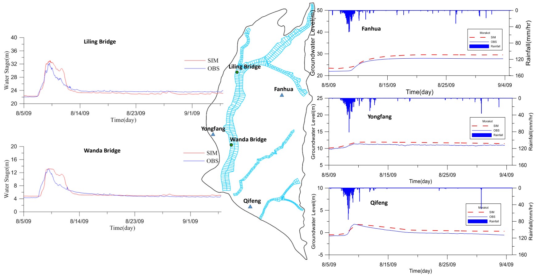
Fig. S2. Calibration results of river stages in the Gaoping River (left) and groundwater levels (right) from August 5 th to September 5 th of 2009.
